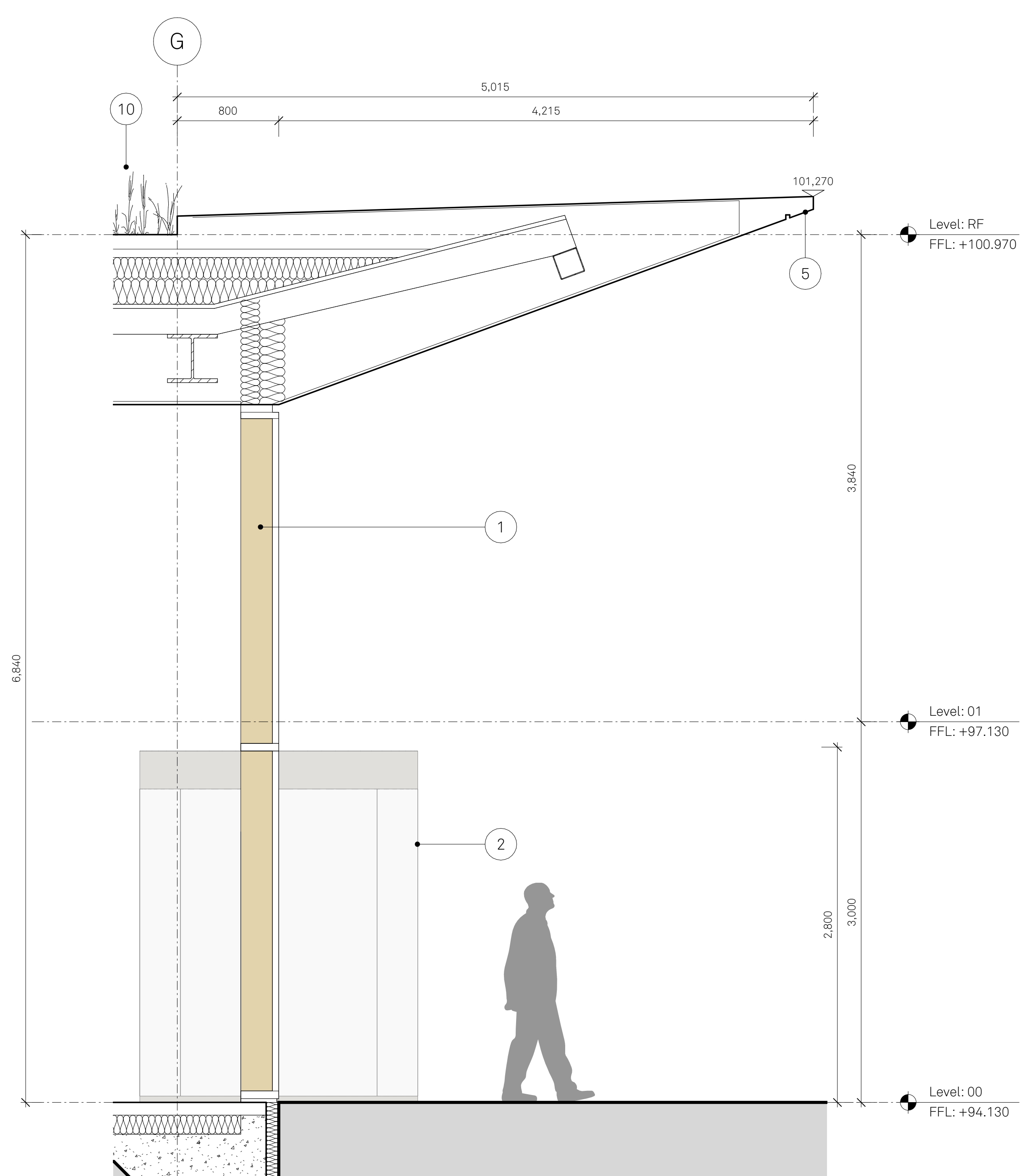
A SECTION THROUGH VILLAGE SQUARE CANOPY
