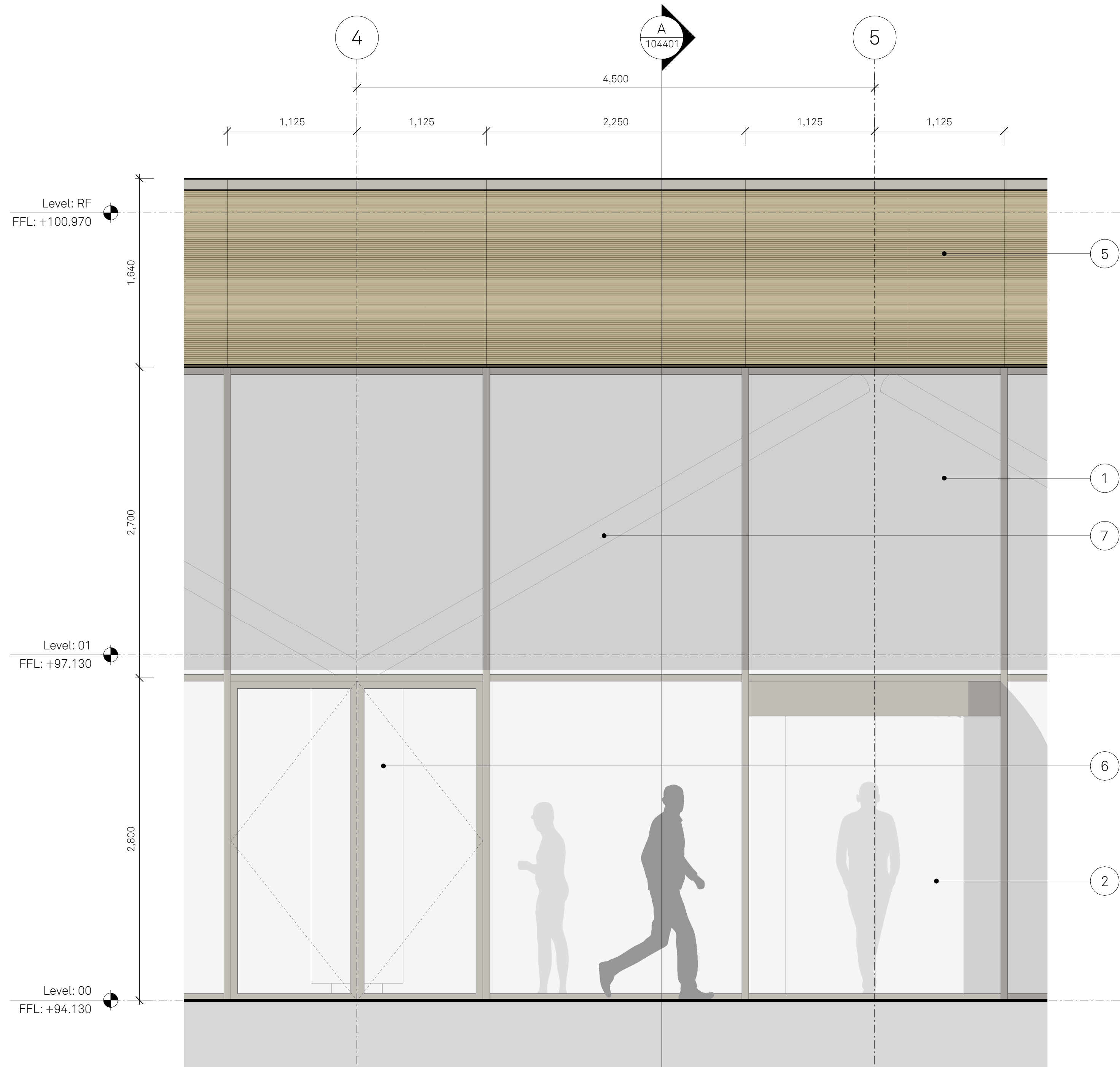
1 DETAIL ELEVATION VILLAGE SQUARE
