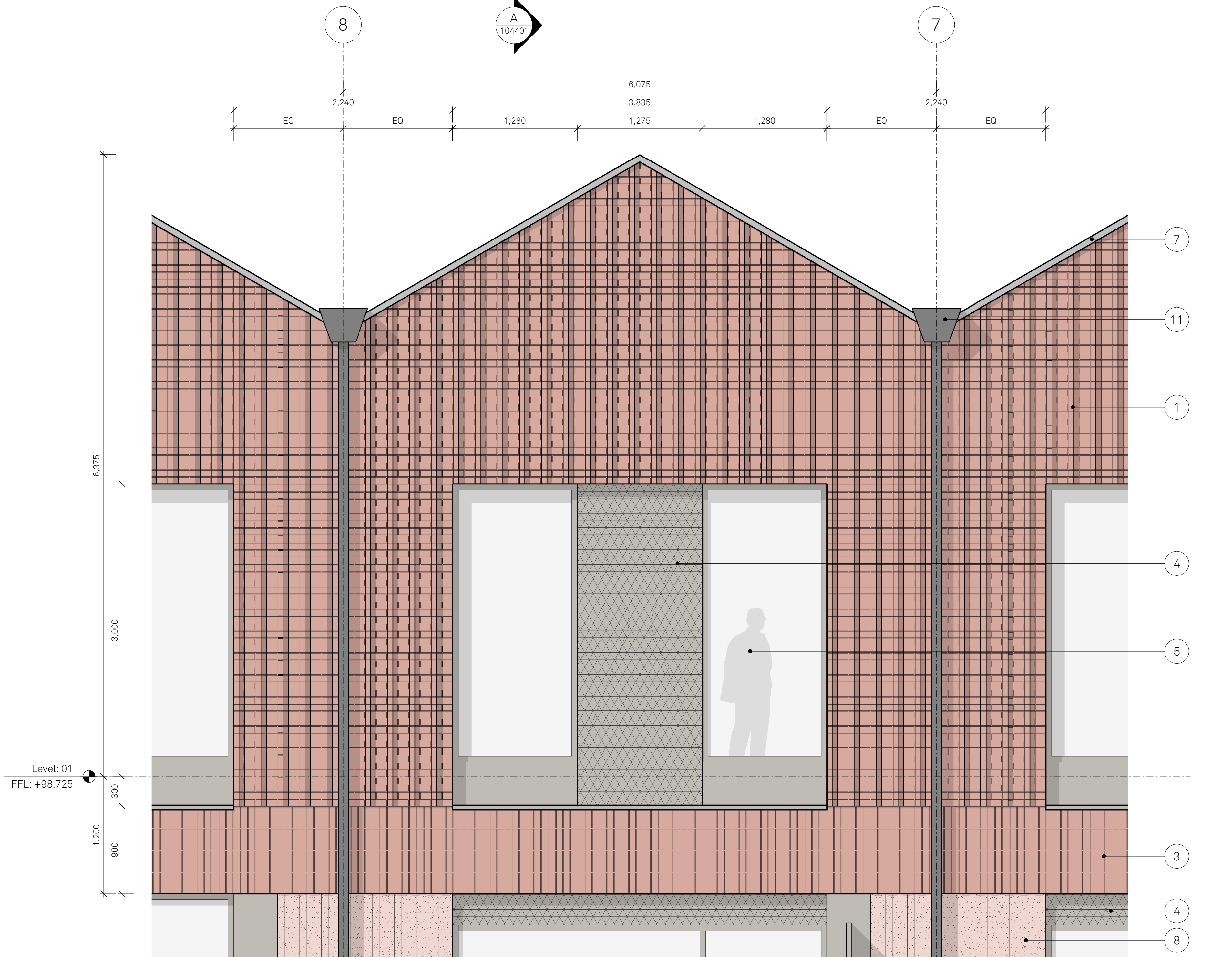
1 DETAIL ELEVATION VILLAGE SQUARE ELEVATION
