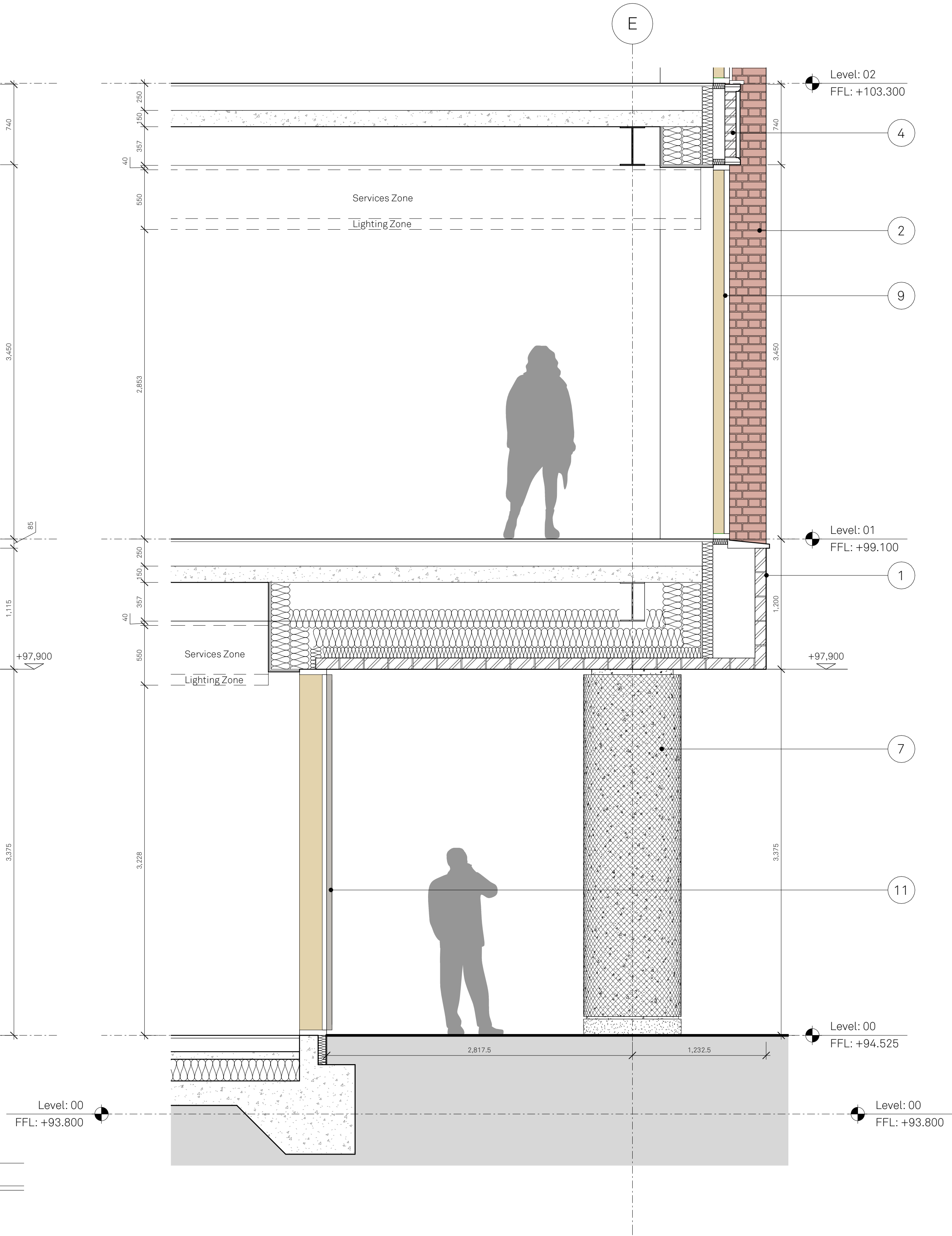
A Study Bay 2 - Section 1 Planning THROUGH CURTAIN WALLING
