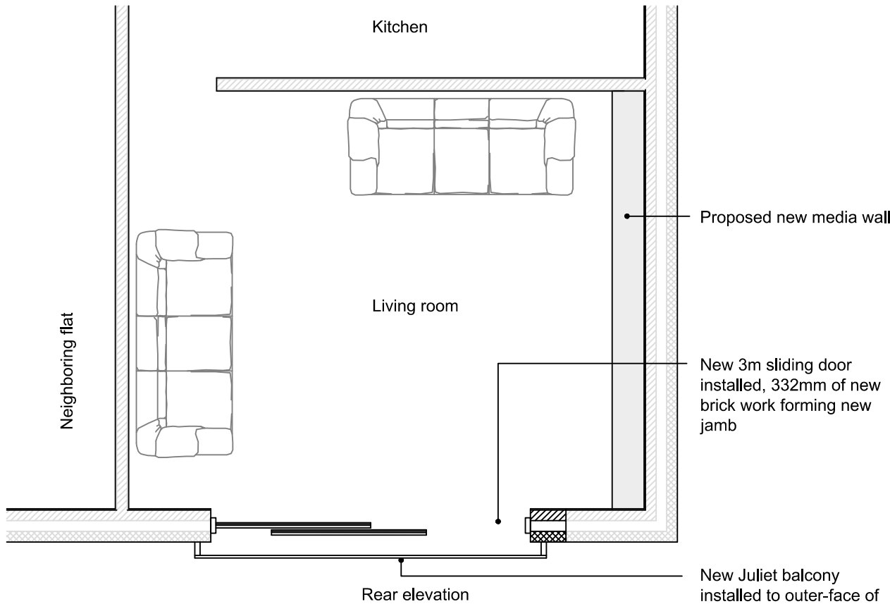
01 Proposed floor plan 1:50
