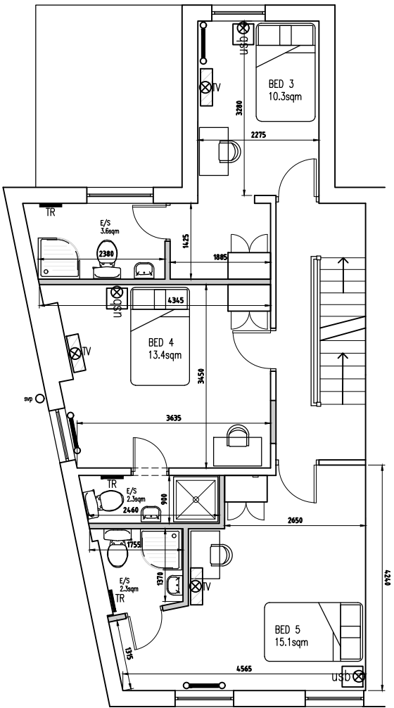
EXISTING FIRST FLOOR PLAN 1:100 @ A3
