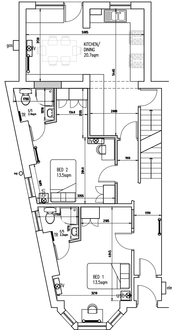
PROPOSED GROUND FLOOR PLAN 1:100 @ A3
