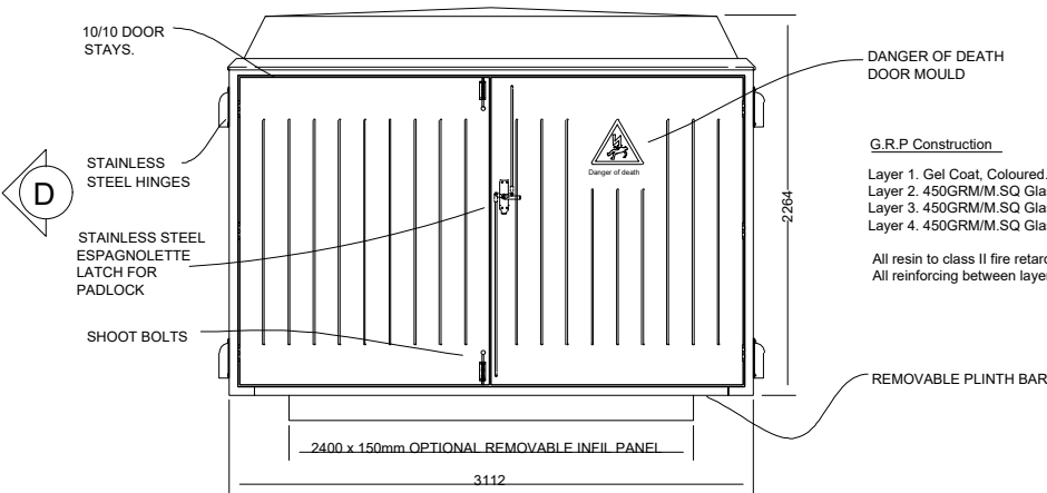
Elevation (B) (rear)
