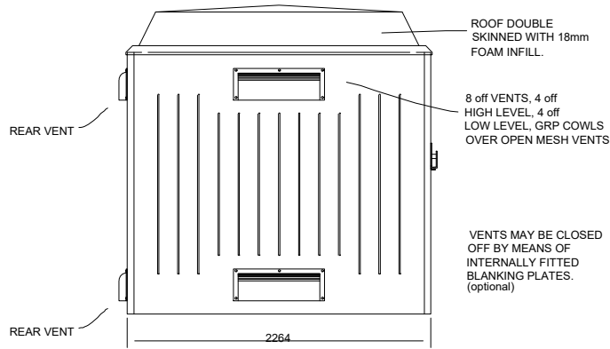
Elevation (C) (l/h side)
