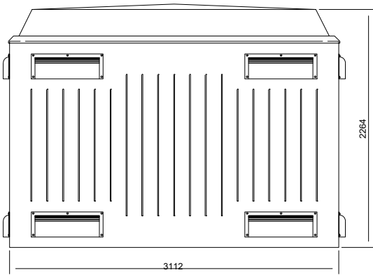
Elevation (B) (rear)
