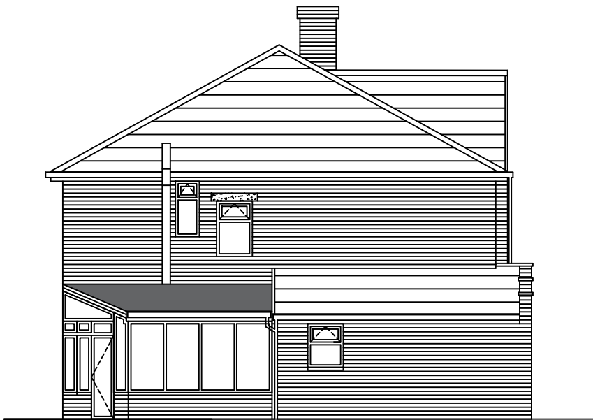
Existing Side Elevation 1:100 @A3
