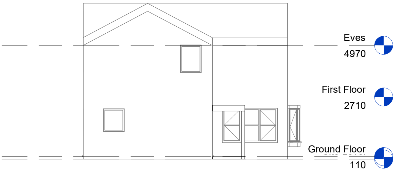
Side 2 Elevation
