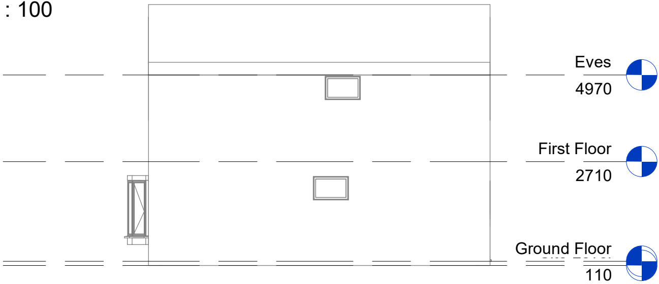
Side 1 Elevation
