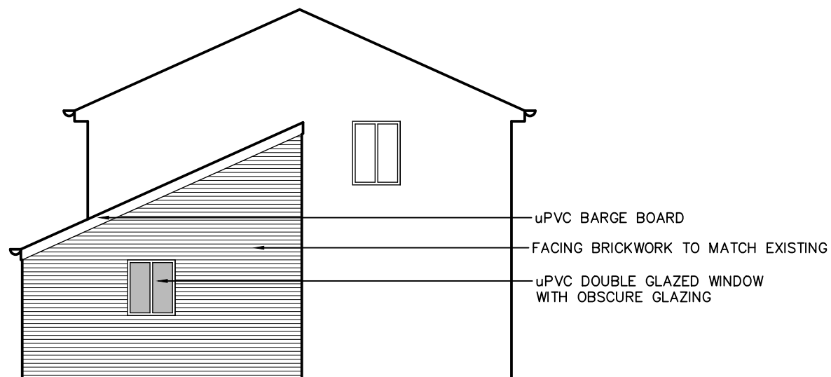
WEST ELEVATION
