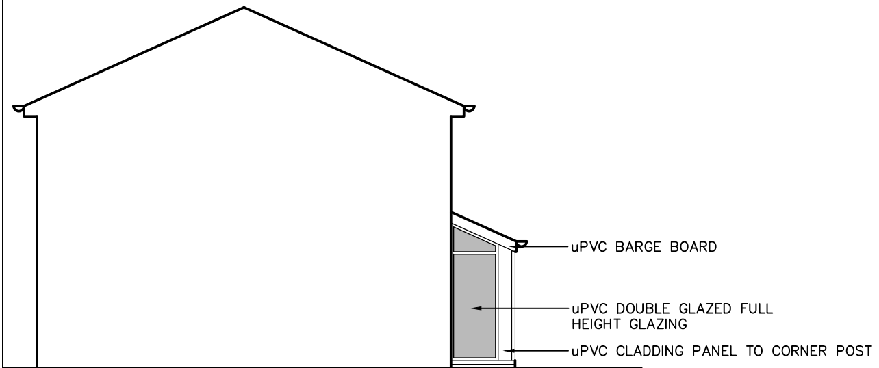
EAST ELEVATION
