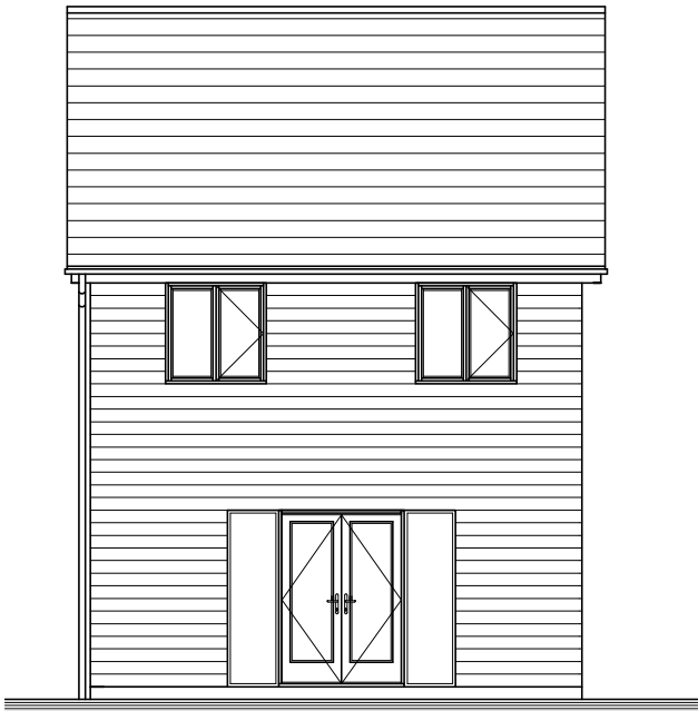
REAR ELEVATION
