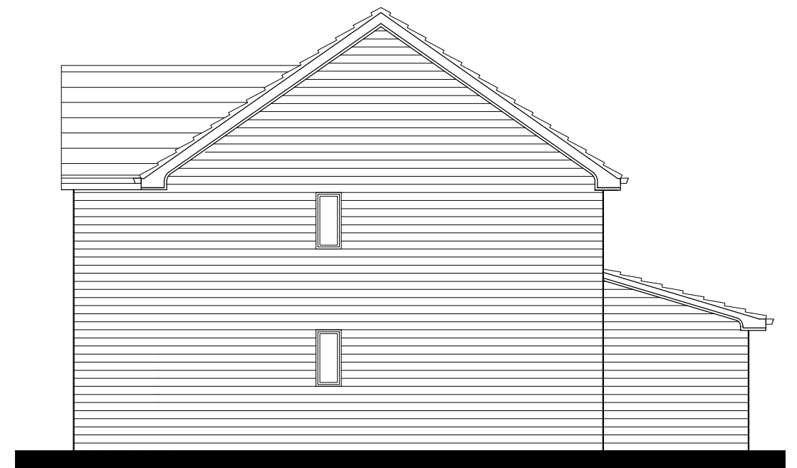
SIDE ELEVATION
