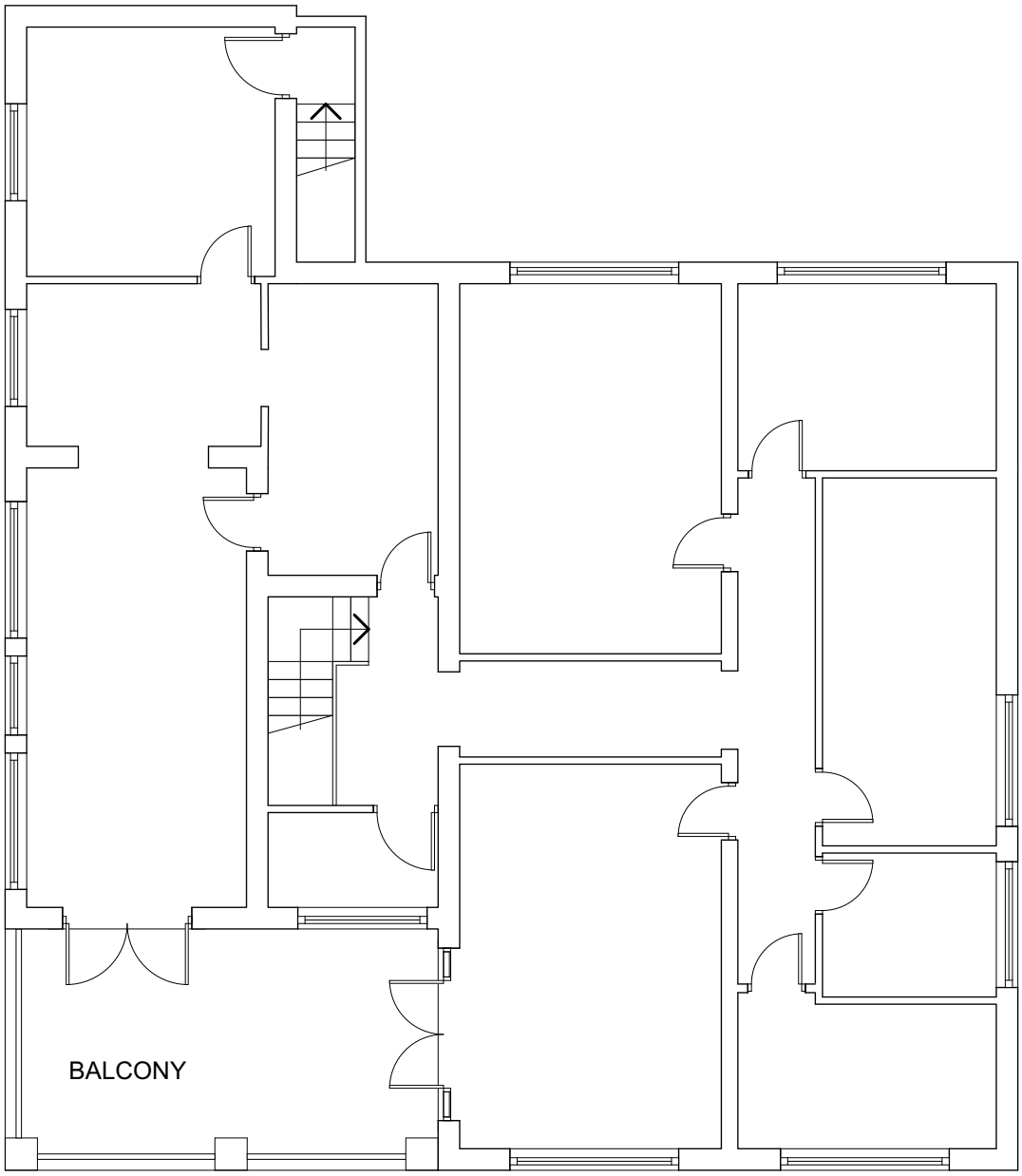
PLAN Existing first floor Scale 1:100 0 1 2 3 4 5m
