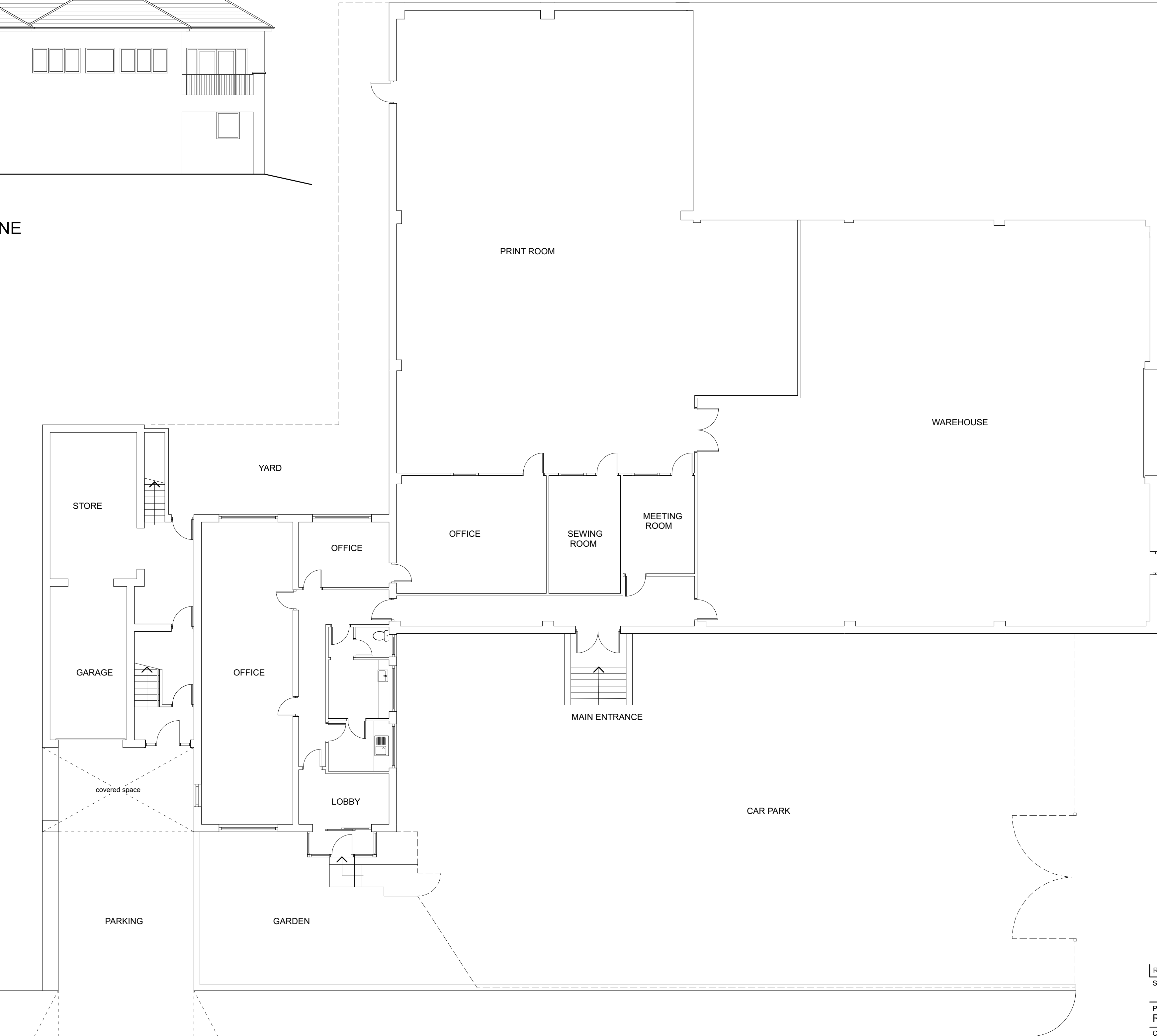
PLAN Existing ground floor Scale 1:100 0 1 2 3 4 5m
