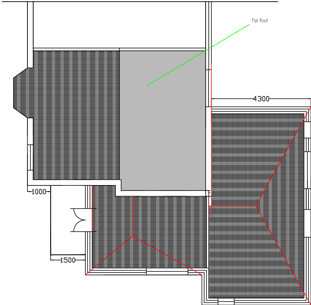
Roof Plan
