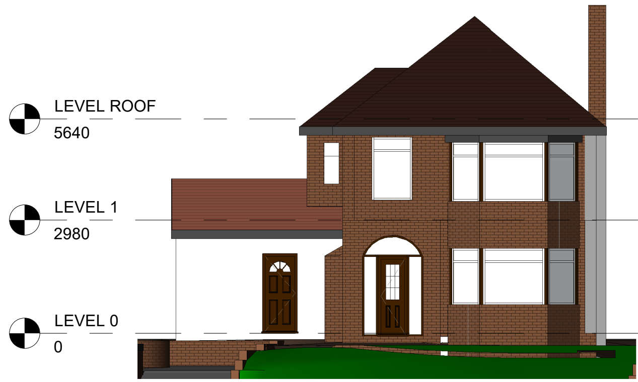
5 Front - Existing 1 : 100
