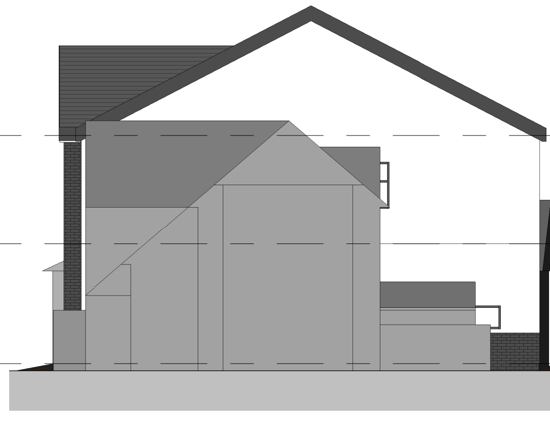
4 Right Side - Proposed 1 : 100
