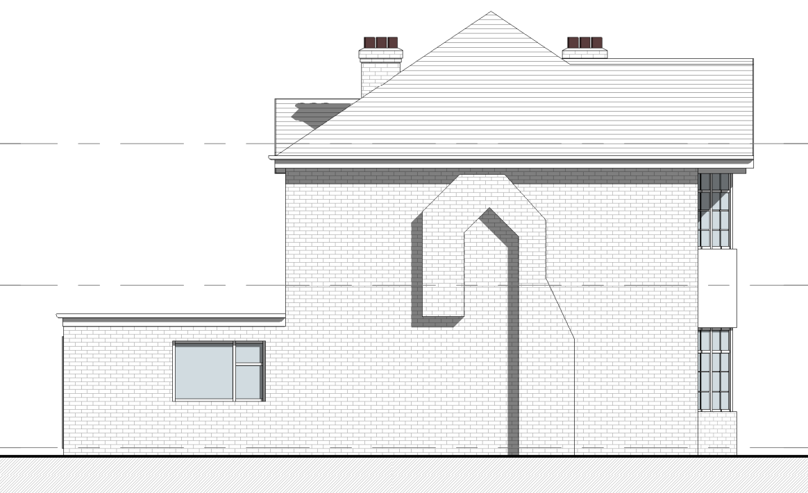
2. Left Side - Existing 1 : 100
