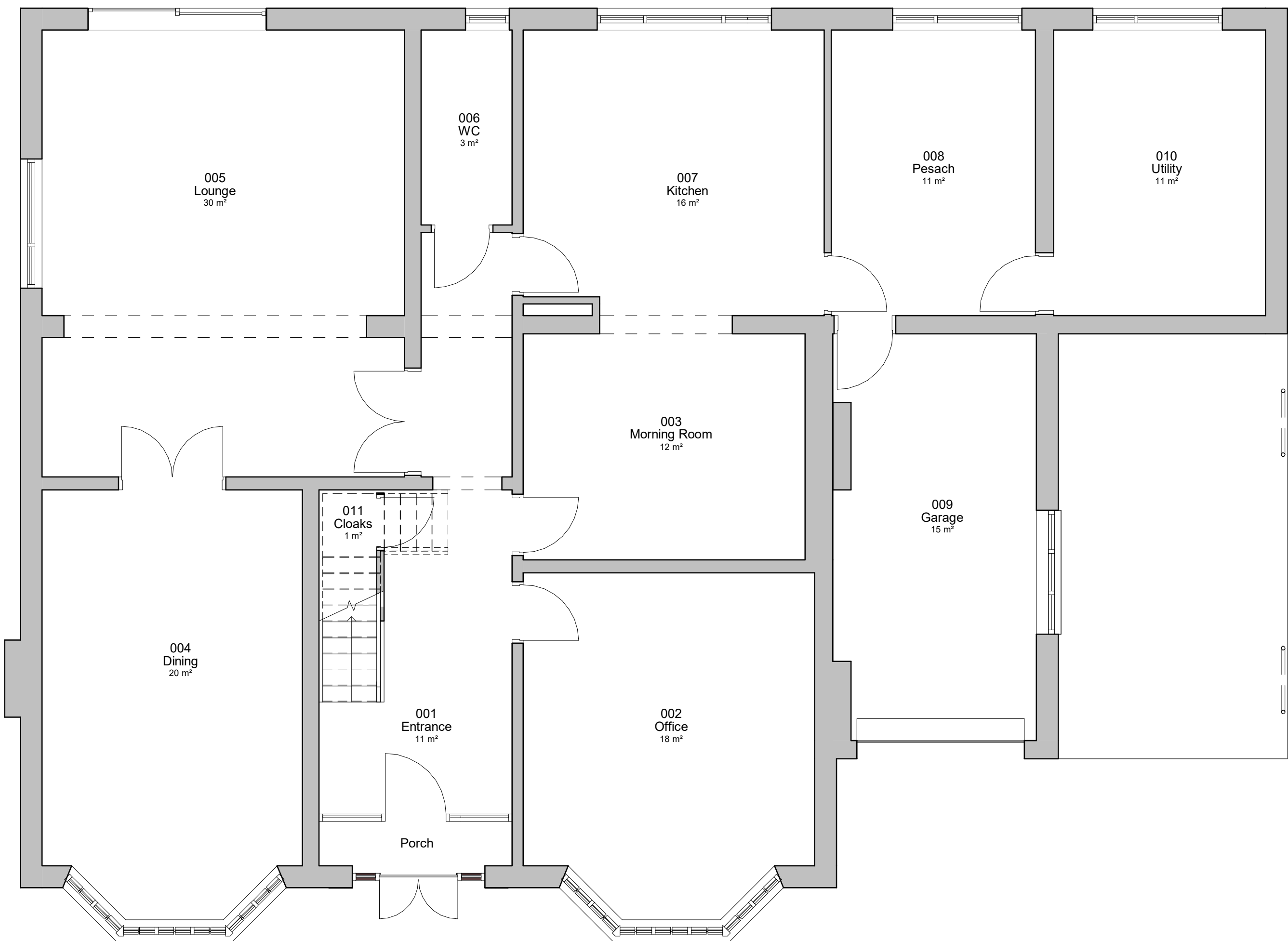
5. Level 0 - GA Existing 1 : 50
