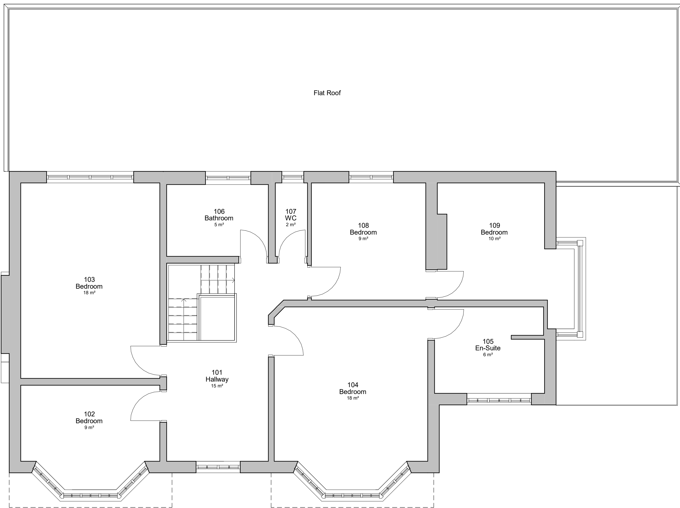
6. Level 1 - GA Existing 1 : 50
