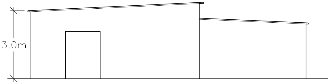
EAST ELEVATION (1:100)
