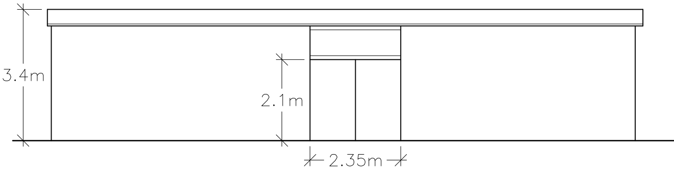
SOUTH ELEVATION (1:100)
