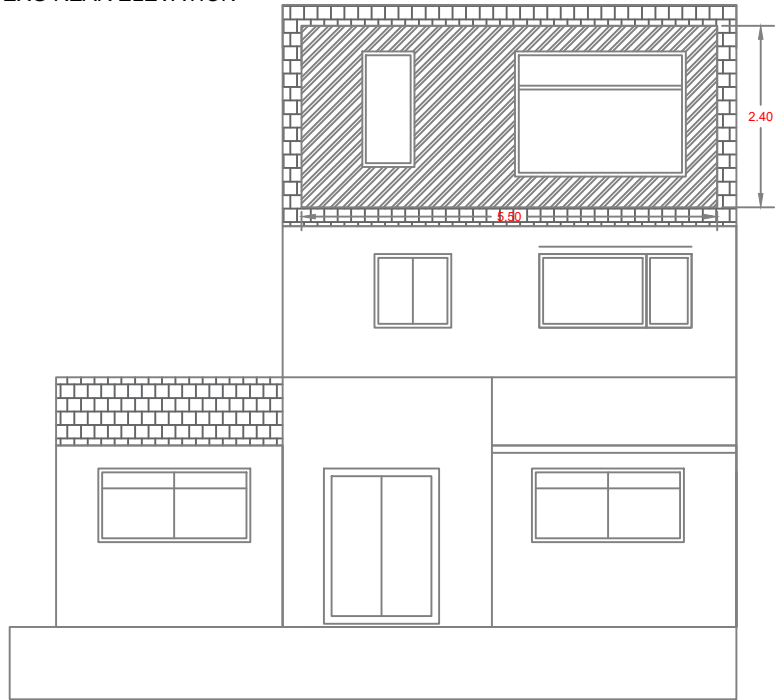
EXG REAR ELEVATION
