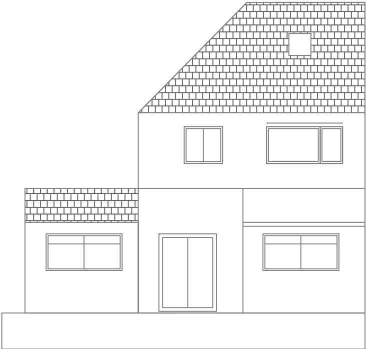
EXG REAR ELEVATION
