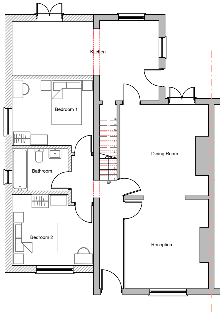
GA Proposed Ground Floor Plan 1:100
