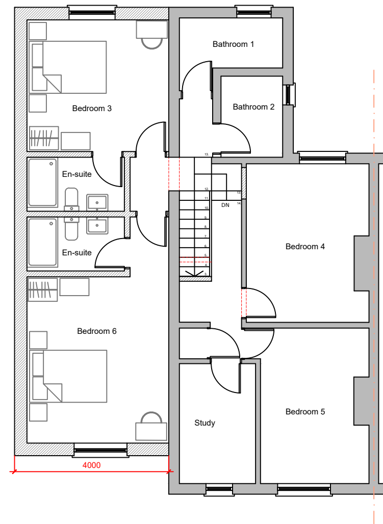
GA Proposed First Floor Plan 1:100
