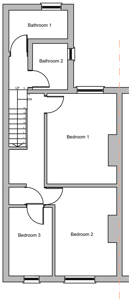
GA Existing First Floor Plan 1:100
