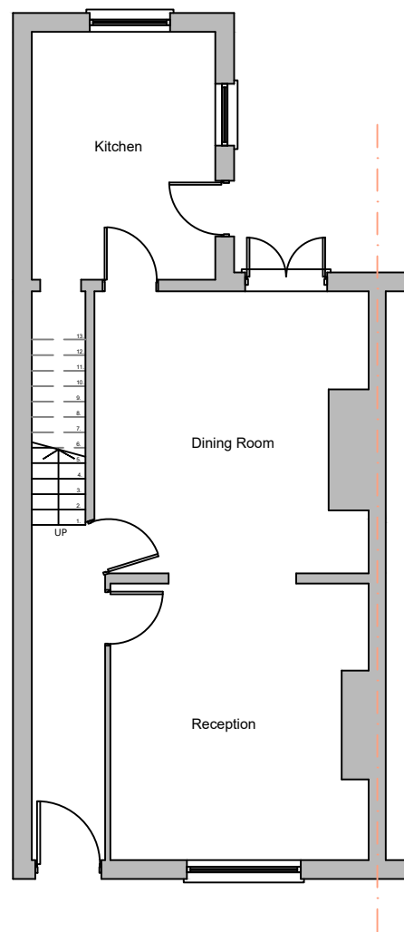
GA Existing Ground Floor Plan 1:100
