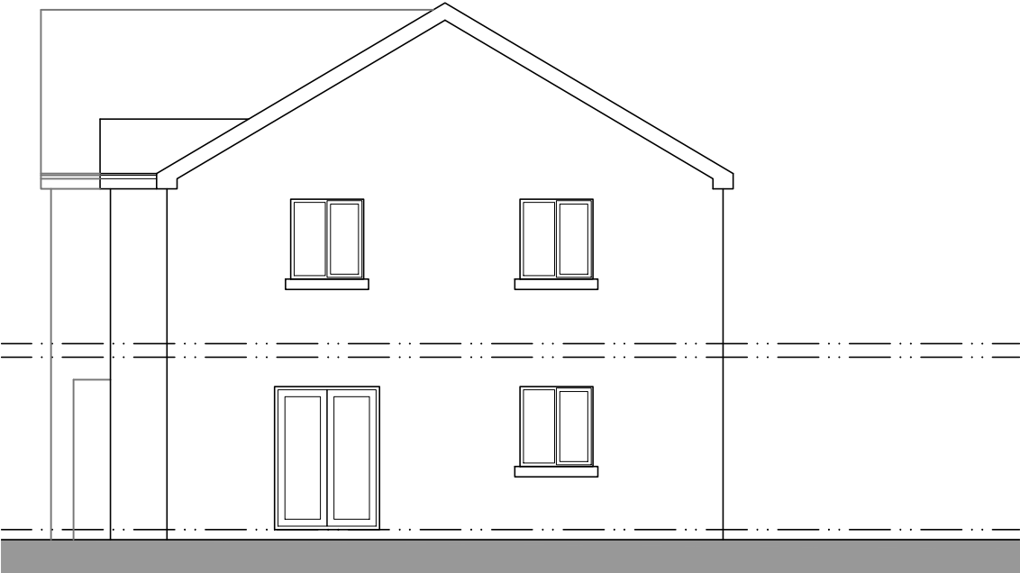
East Facing Side Elevation
