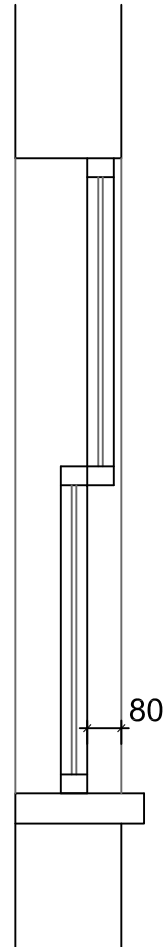
SASH WINDOW SECTION 1:20 @ A4
