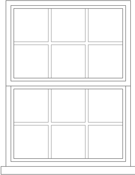
SASH WINDOW ELEVATION 1:20 @ A4
