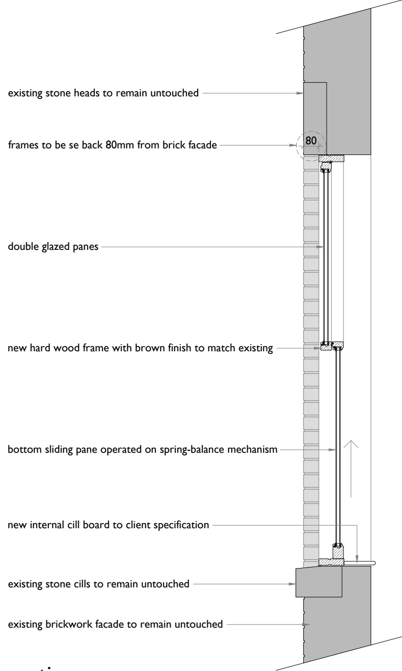
section
