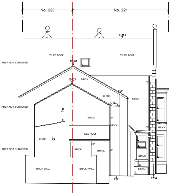
Rear Elevation
