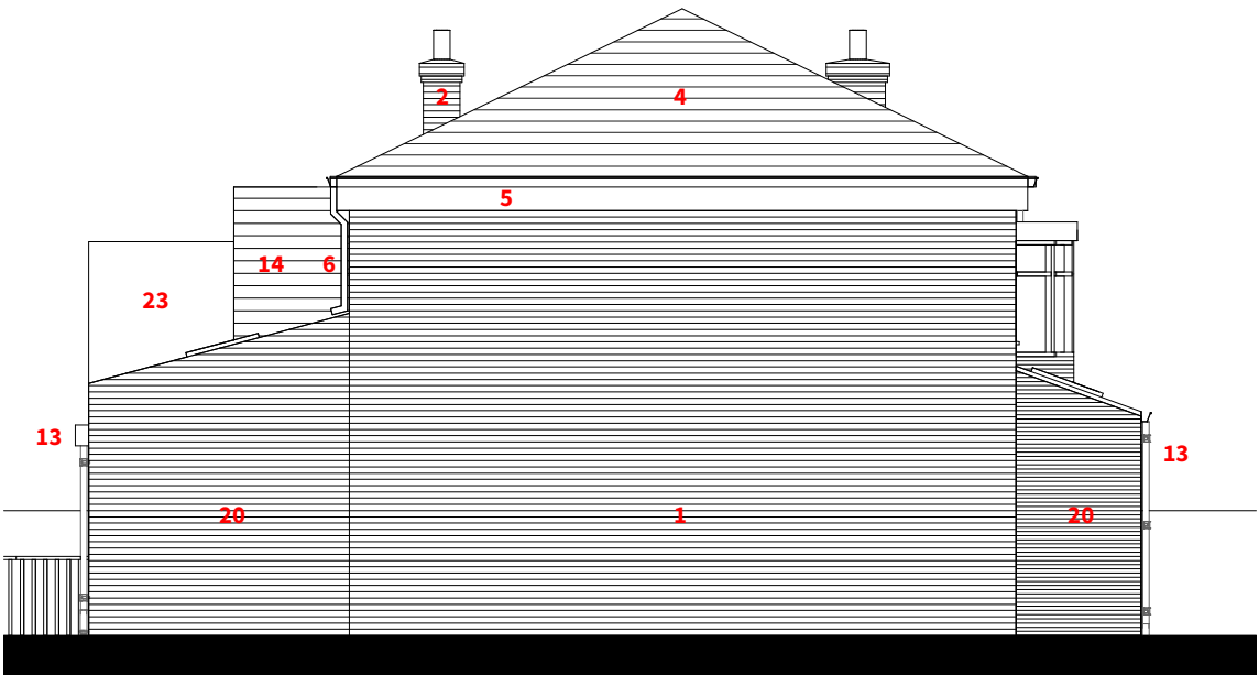
Proposed Side B Elevation 1:100 / A3
