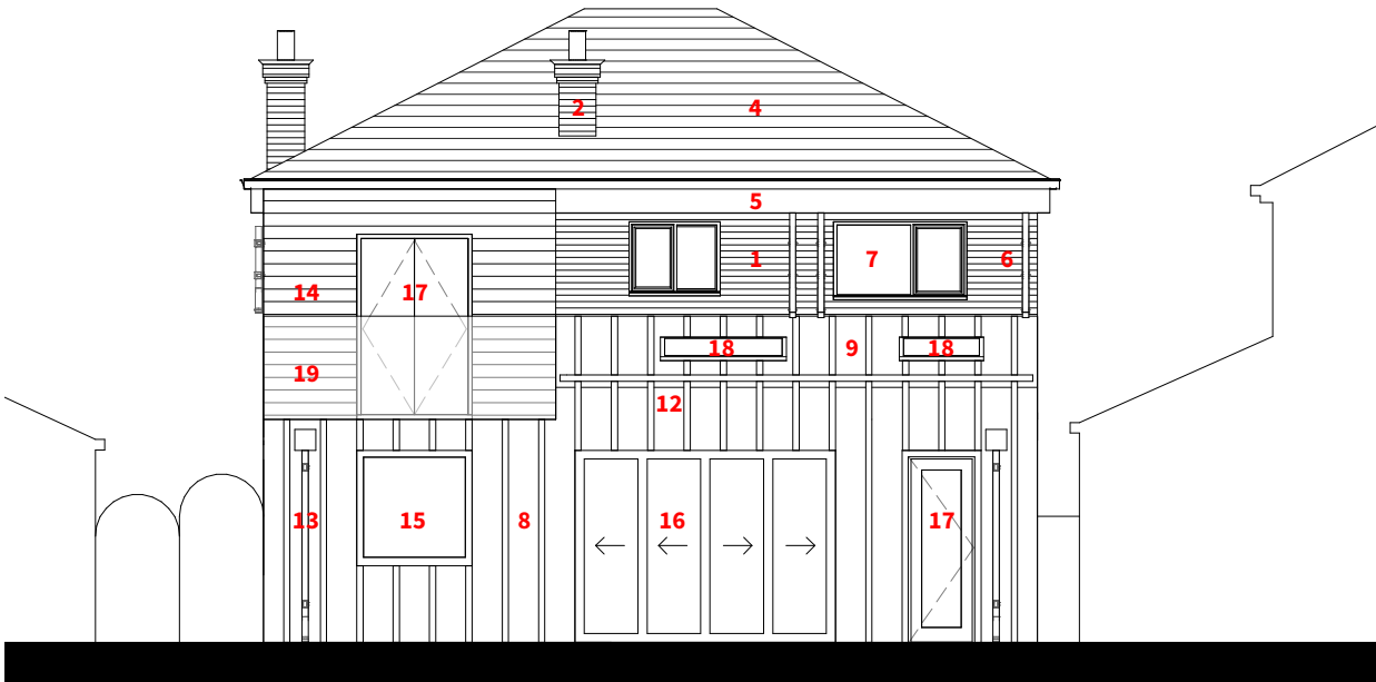
Proposed Rear Elevation 1:100 / A3
