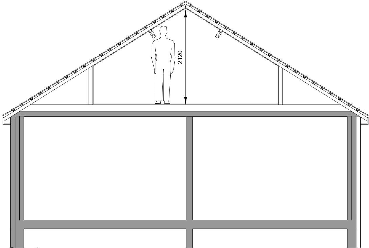
Existing Cross Section
