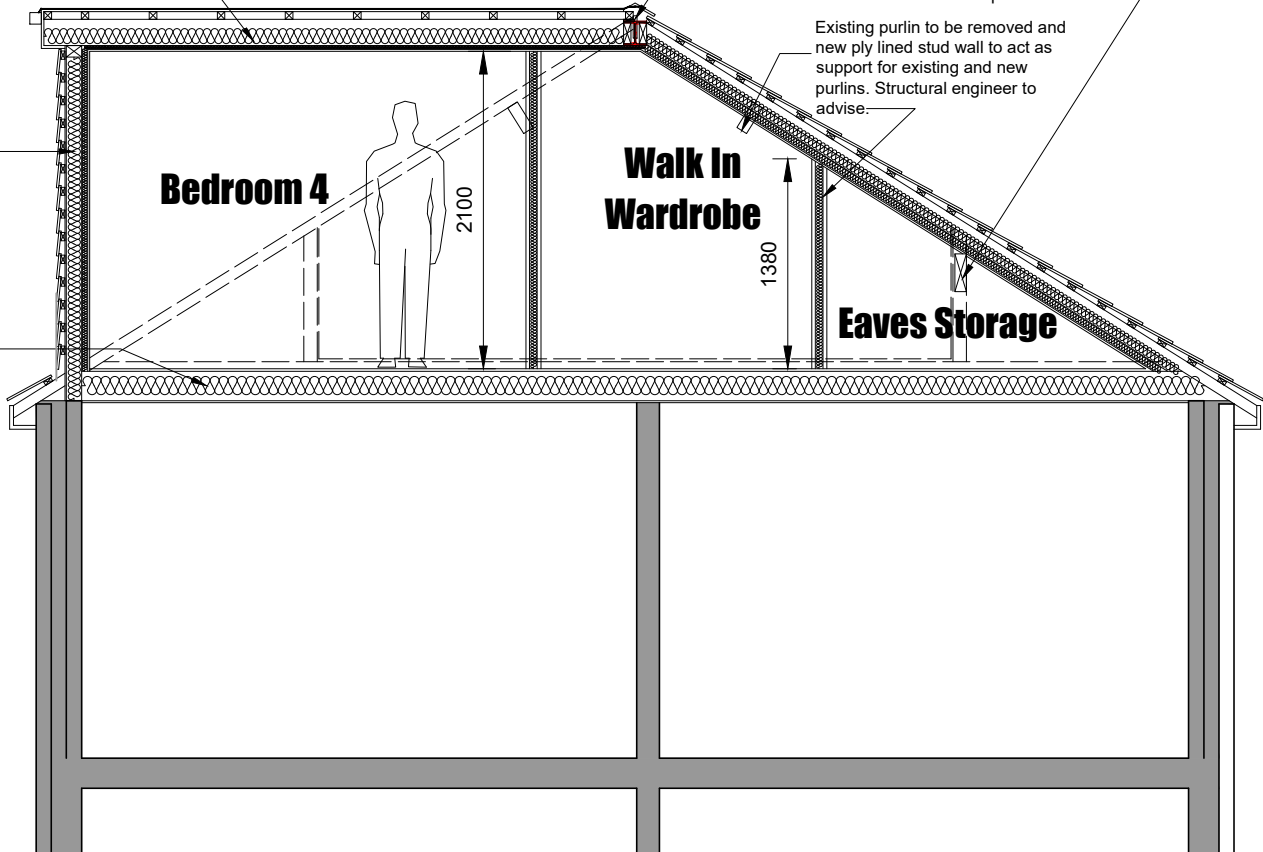
Proposed Cross Section
