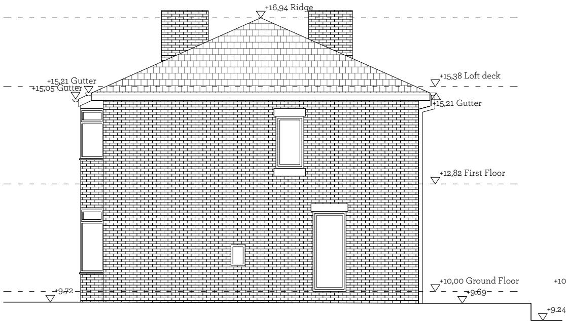
Northern Elevation
