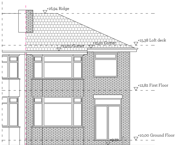
Eastern Elevation (Front)
