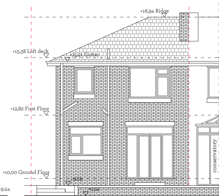
Western Elevation
