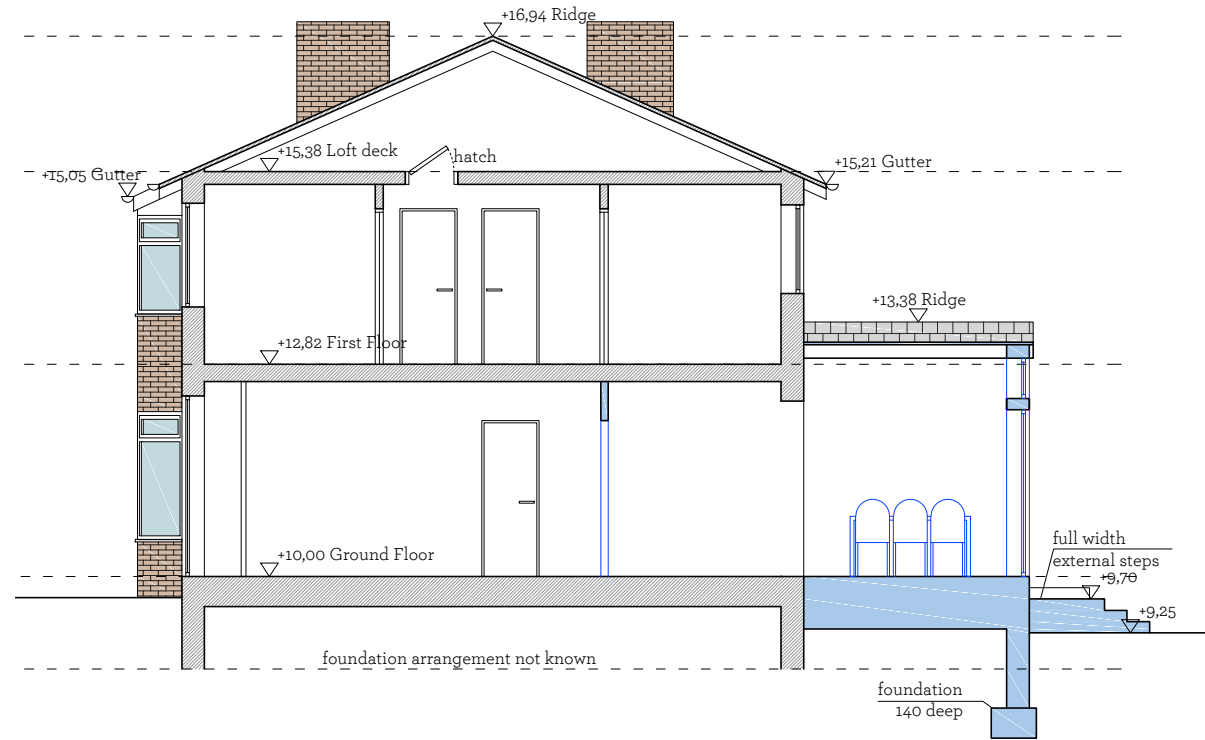
Proposed Section A
