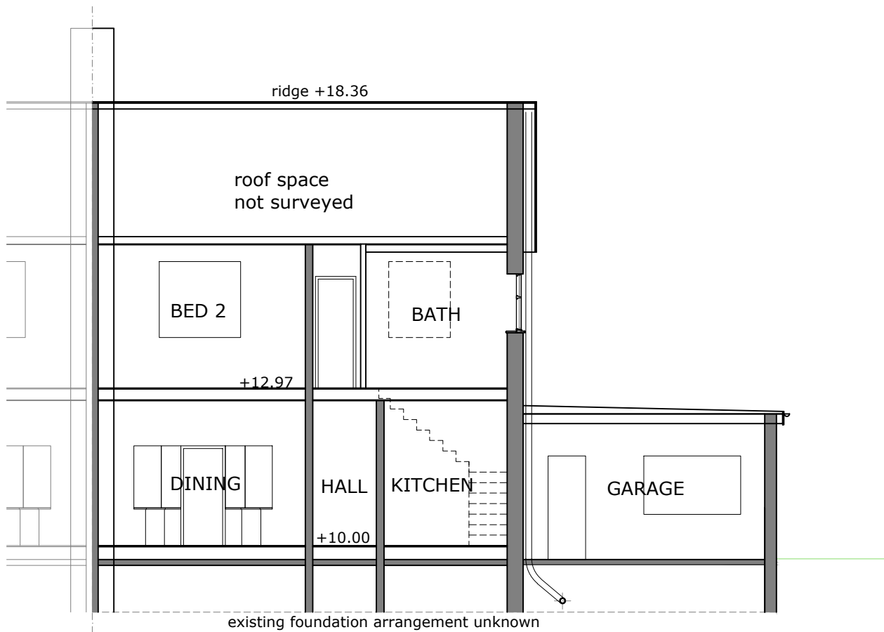
CROSS SECTION
