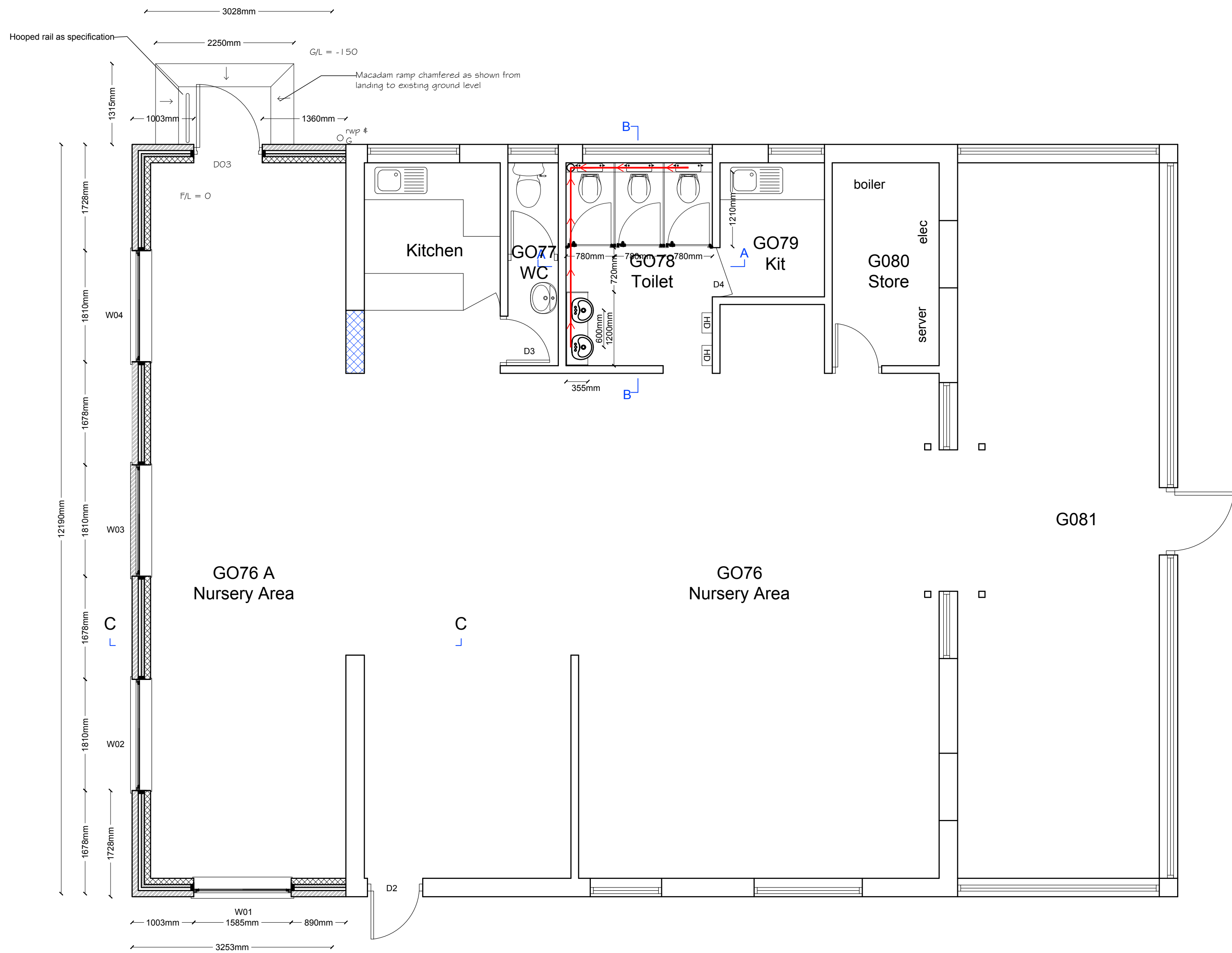
Proposed Layout Plan 1:50 @A1
