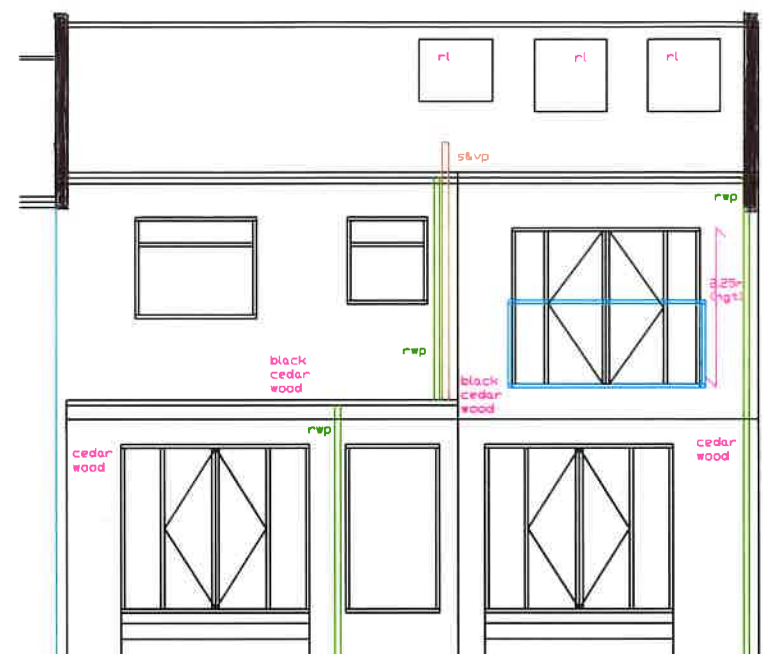
PROPOSED REAR VIEW 1:100
