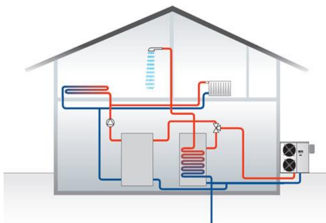
Figure 11 - Principles of an ASHP system
