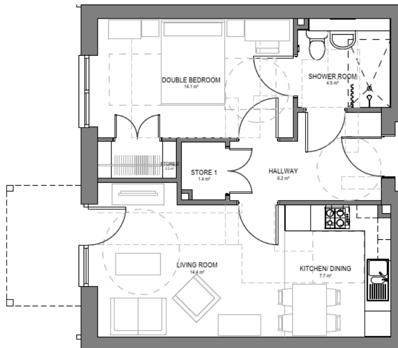
Figure 4 – Proposed APT_T1 Floor Plans
