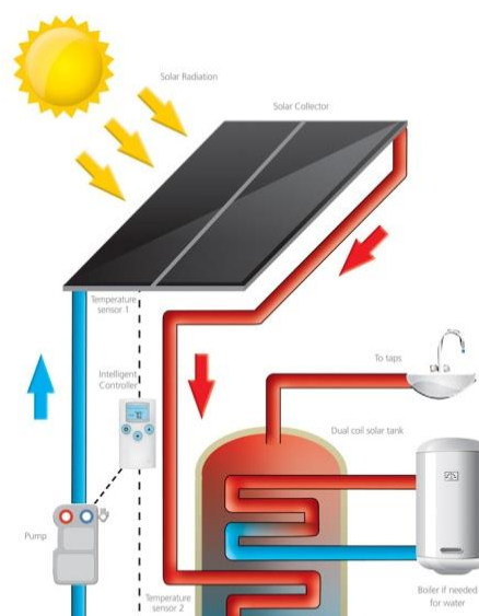
Figure 9 - The principles of a solar thermal system
