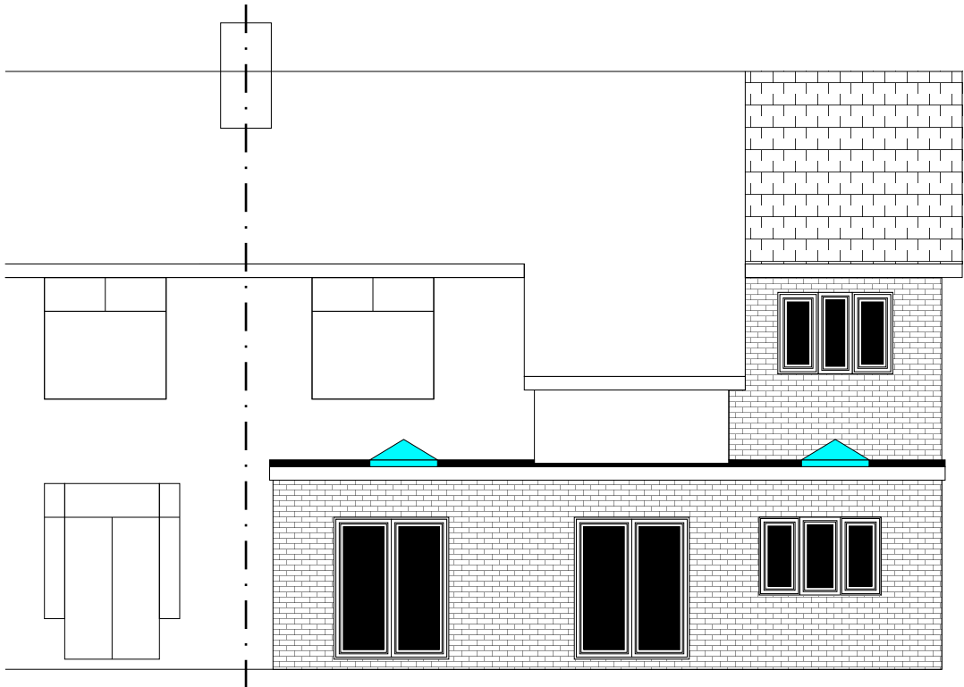
EXISTING EAST REAR ELEVATION
