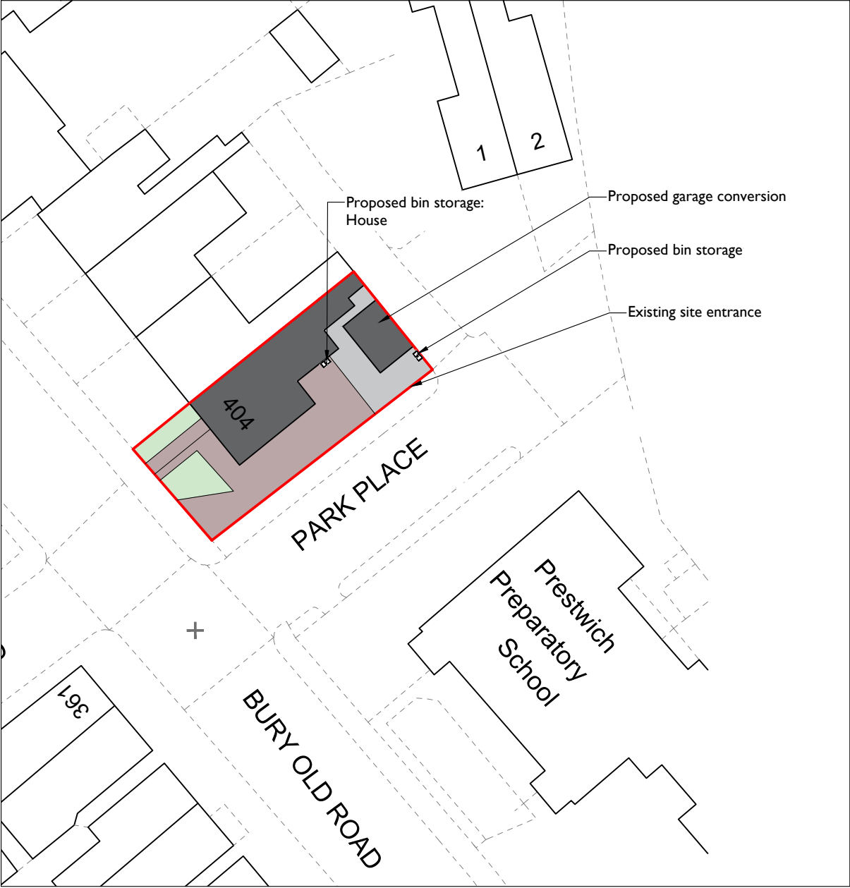
Proposed Block Plan: 1:500 at A3
