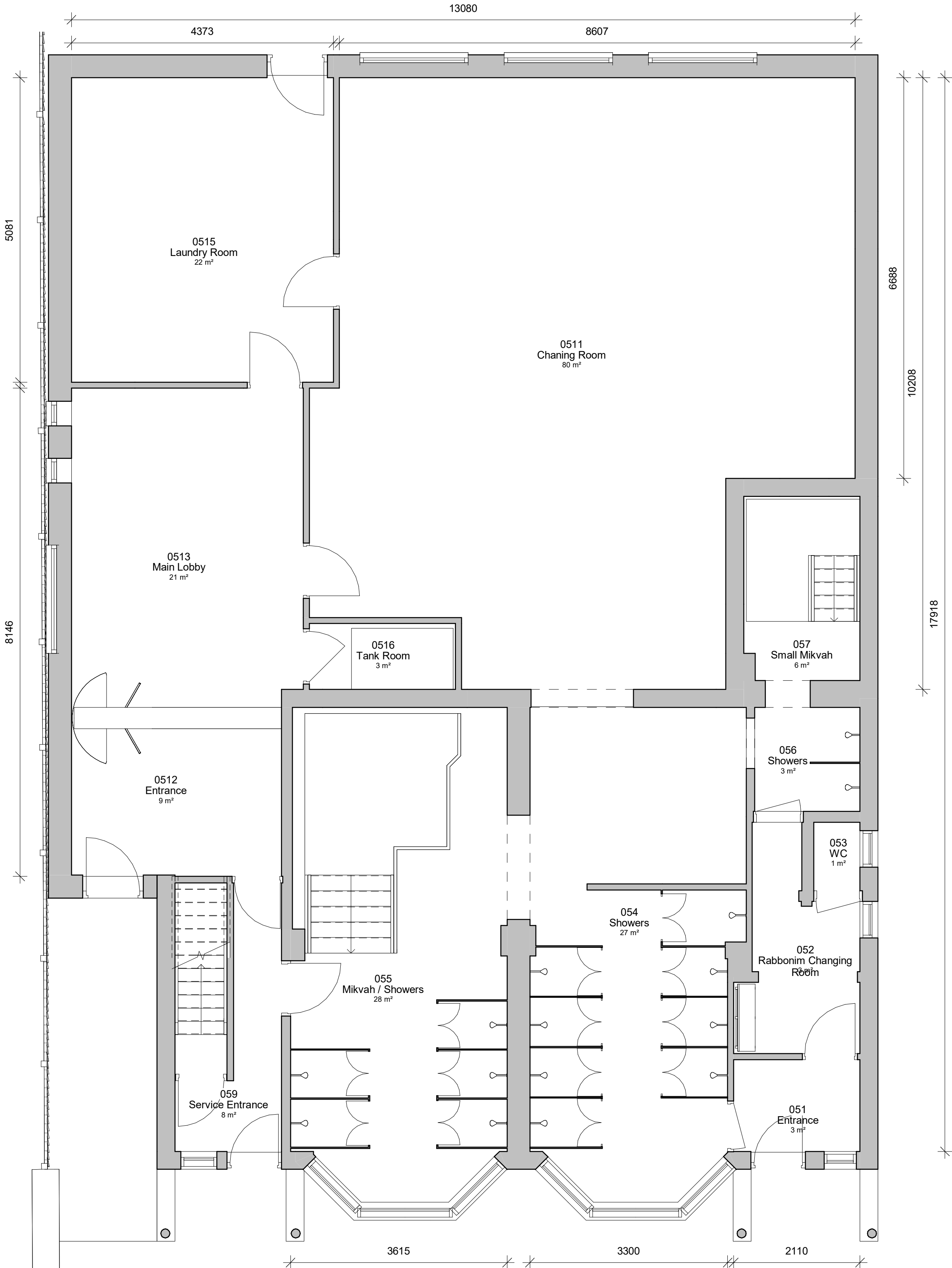
5. Level 0 - GA Proposed
