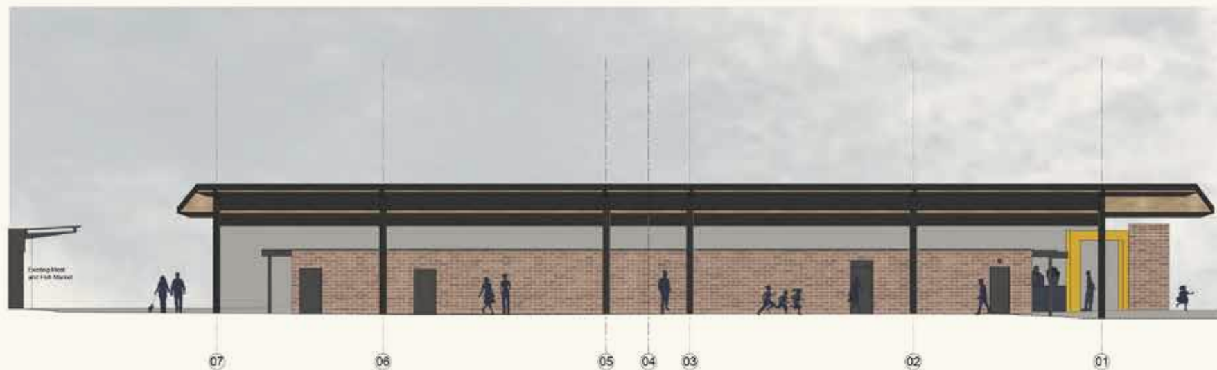
ELEVATION 2 - CANOPY ROOF 1
