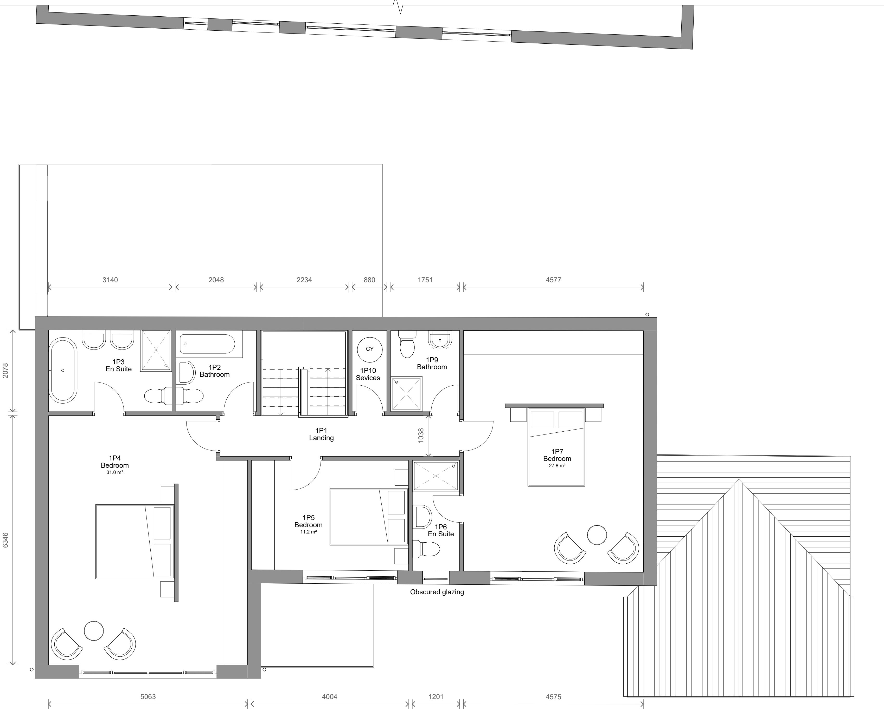
1 Level 1 - Proposed 1 : 50
