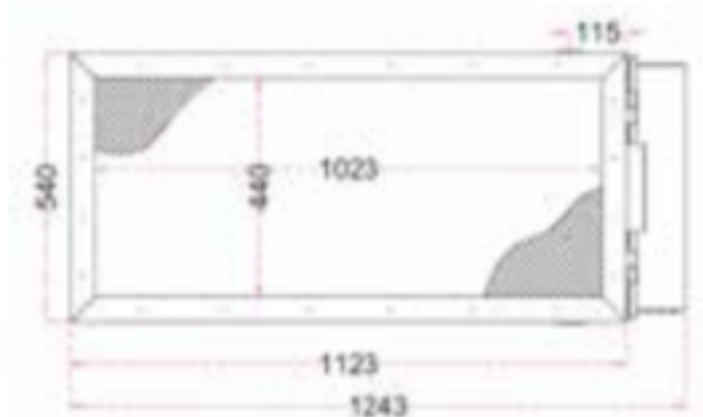
Air Discharge View
