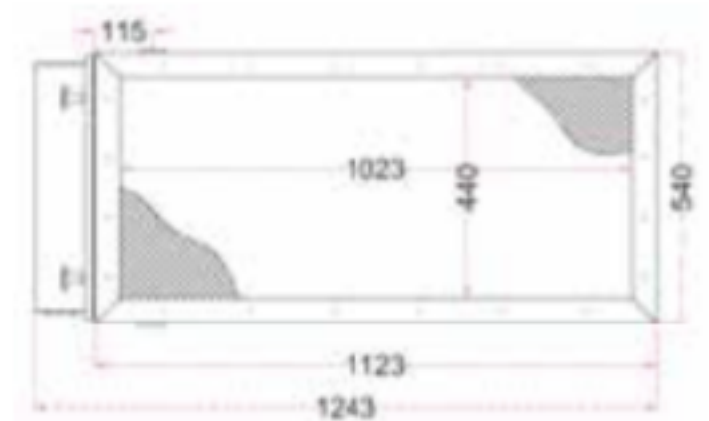
Air Intake View
