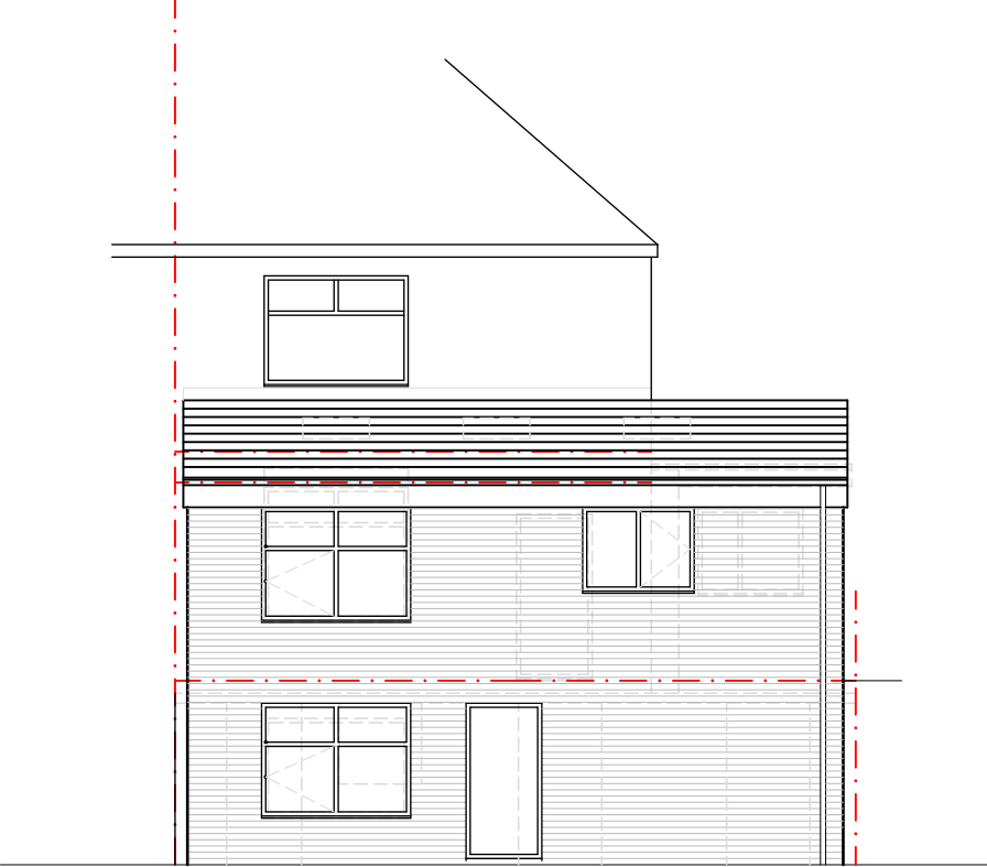
REAR ELEVATION 1:100
