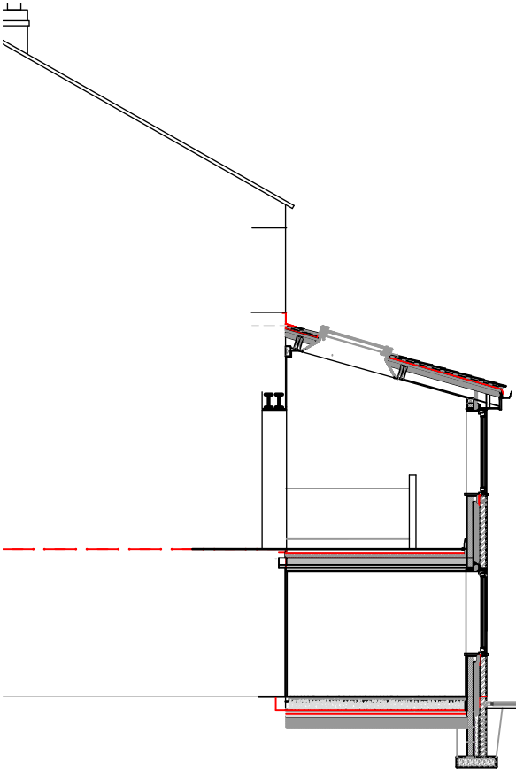
GA SECTION A-A 1:100 Refer also to 1:20 section.
