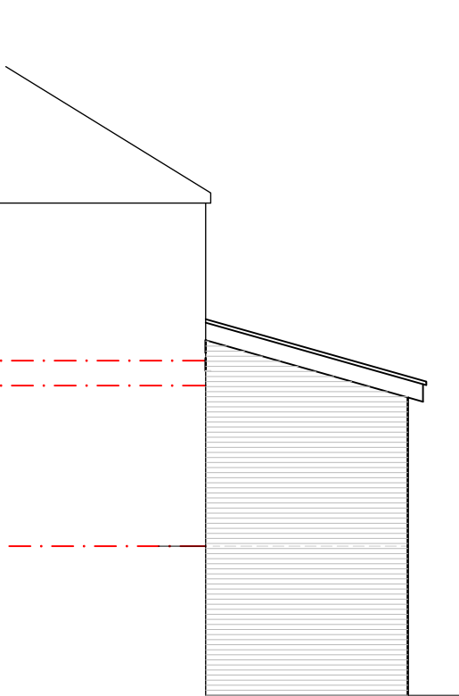
REAR ELEVATION 1:100
