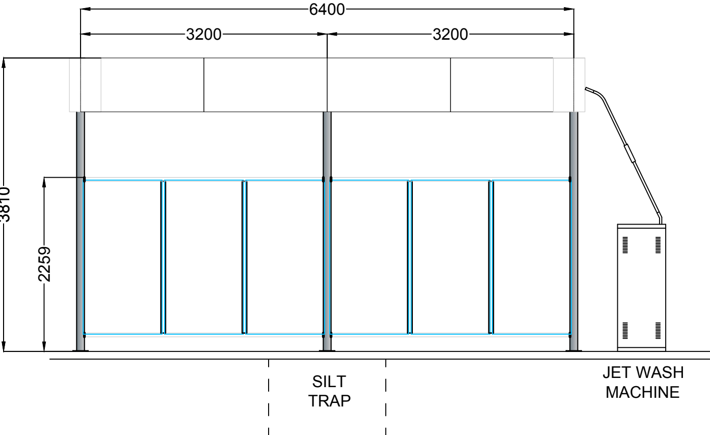
JET WASH BAY ELEVATION D - Scale 1:50
