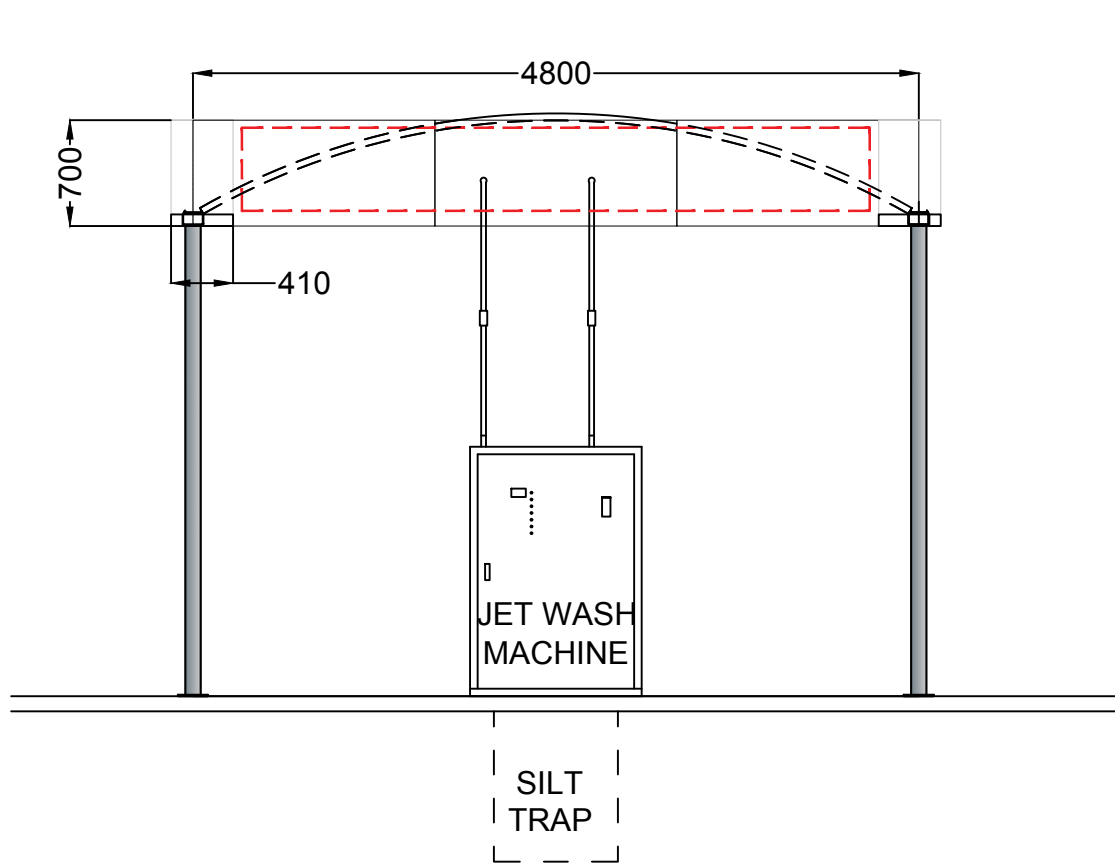
JET WASH BAY ELEVATION A - Scale 1:50
