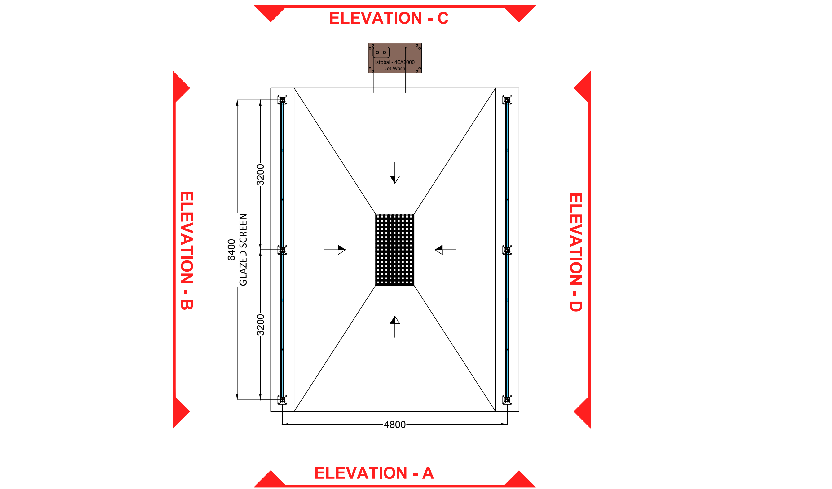
JET WASH BAY LAYOUT - Scale 1:50
