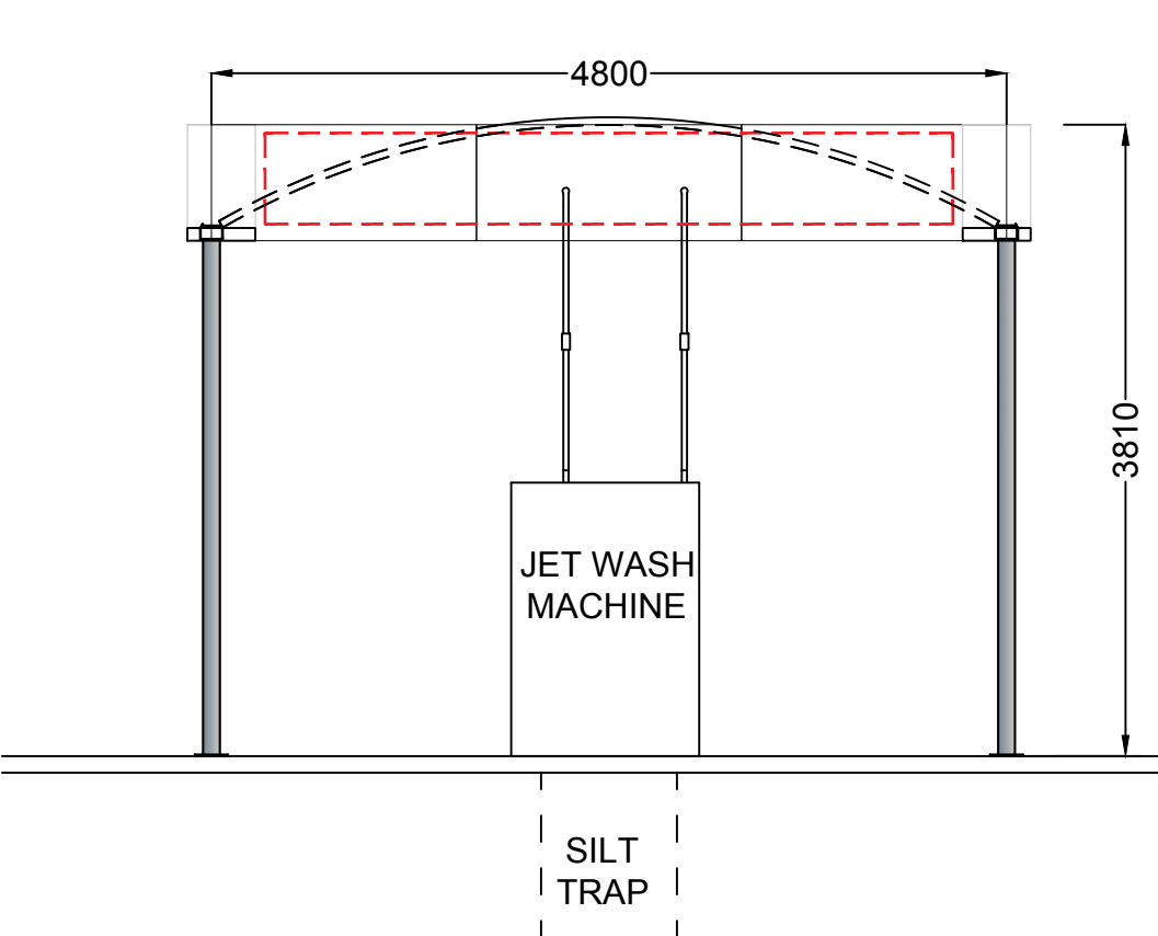
JET WASH BAY ELEVATION C - Scale 1:50
