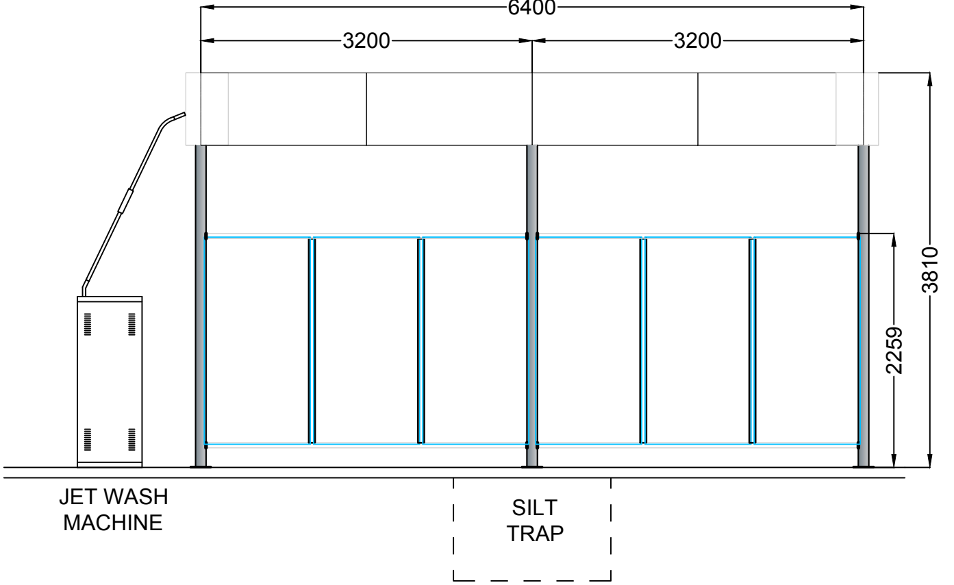
JET WASH BAY ELEVATION B - Scale 1:50
