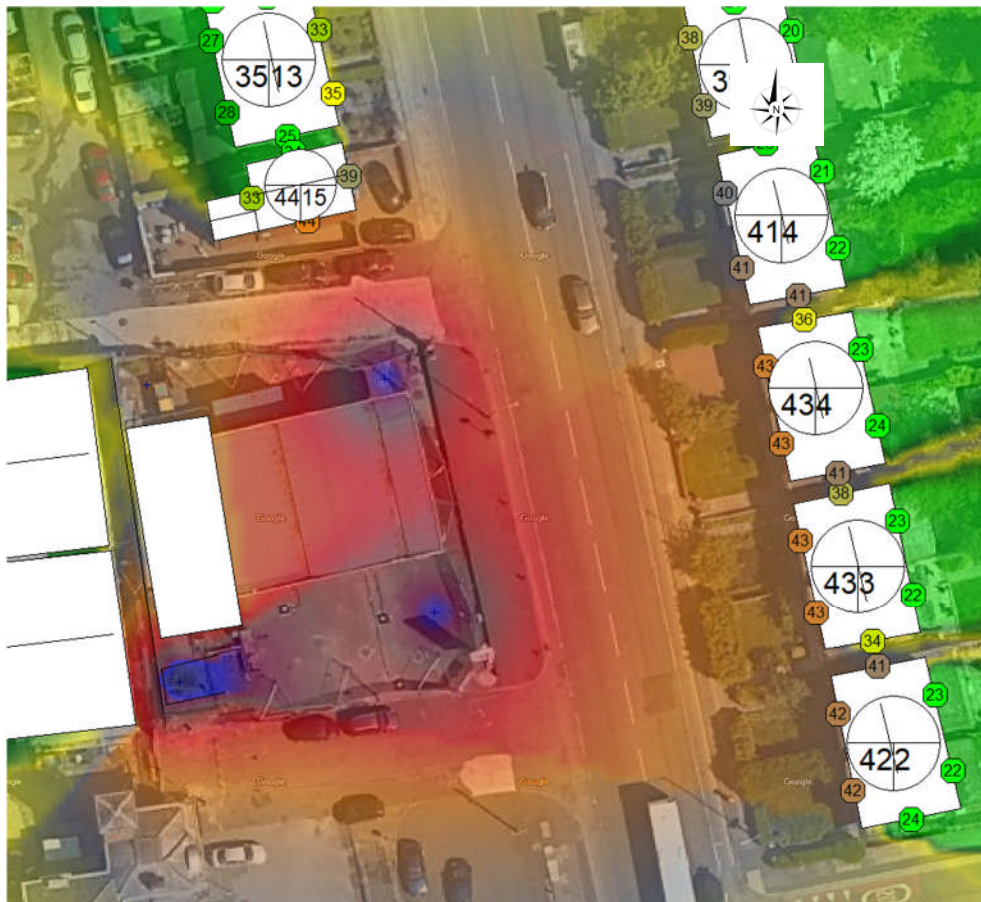
Figure 3: Specific Noise Levels as calculated: (Substation +air,water,vacuum stations + jet wash bay operating / Substation only) – L_{Aeq,T}
