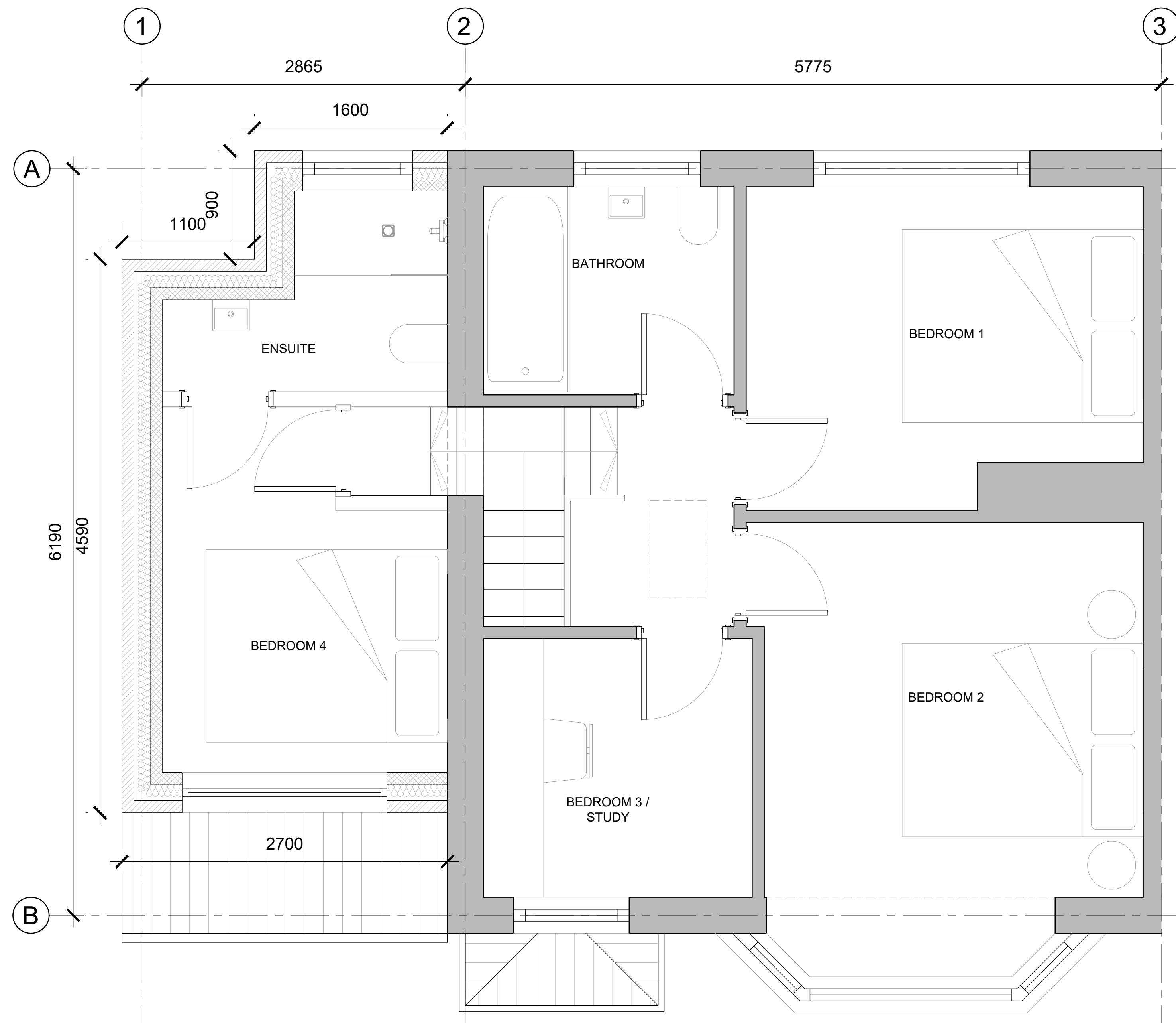
PROPOSED FIRST FLOOR
