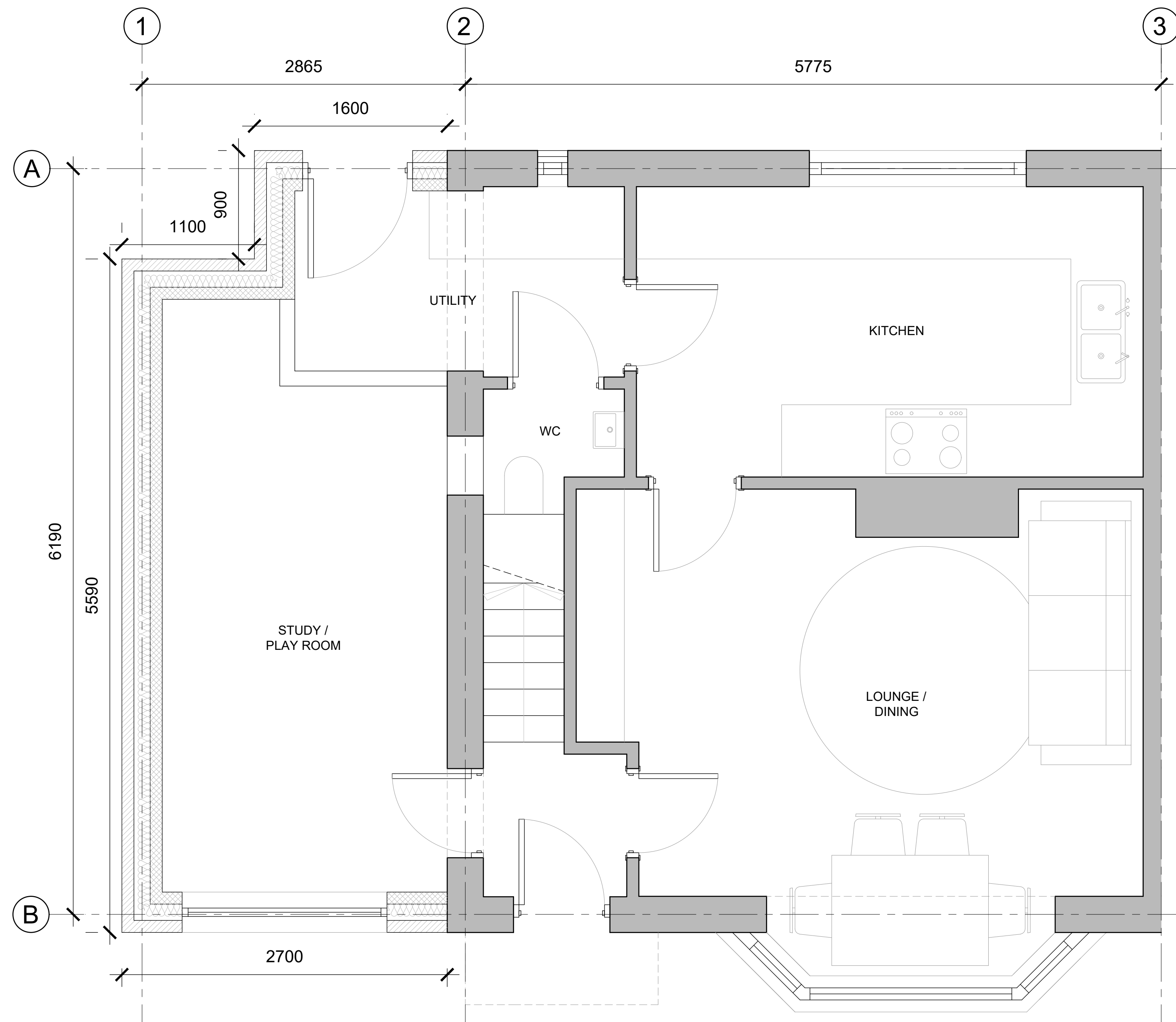
PROPOSED GROUND FLOOR
