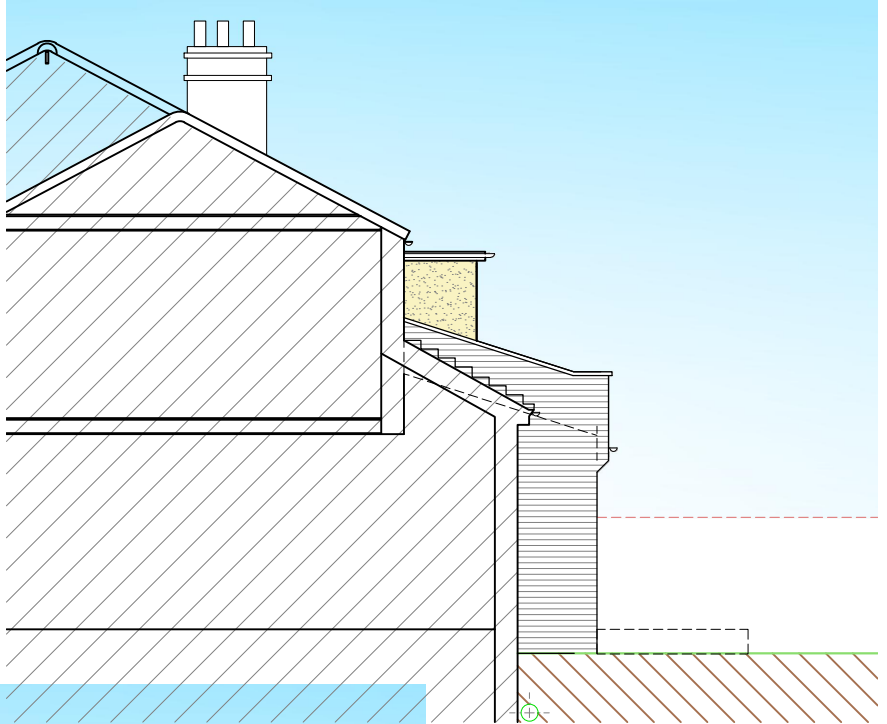
WEST ELEVATION TO NEIGHBOUR
