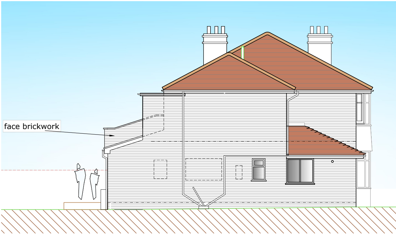
EAST (SIDE) ELEVATION
