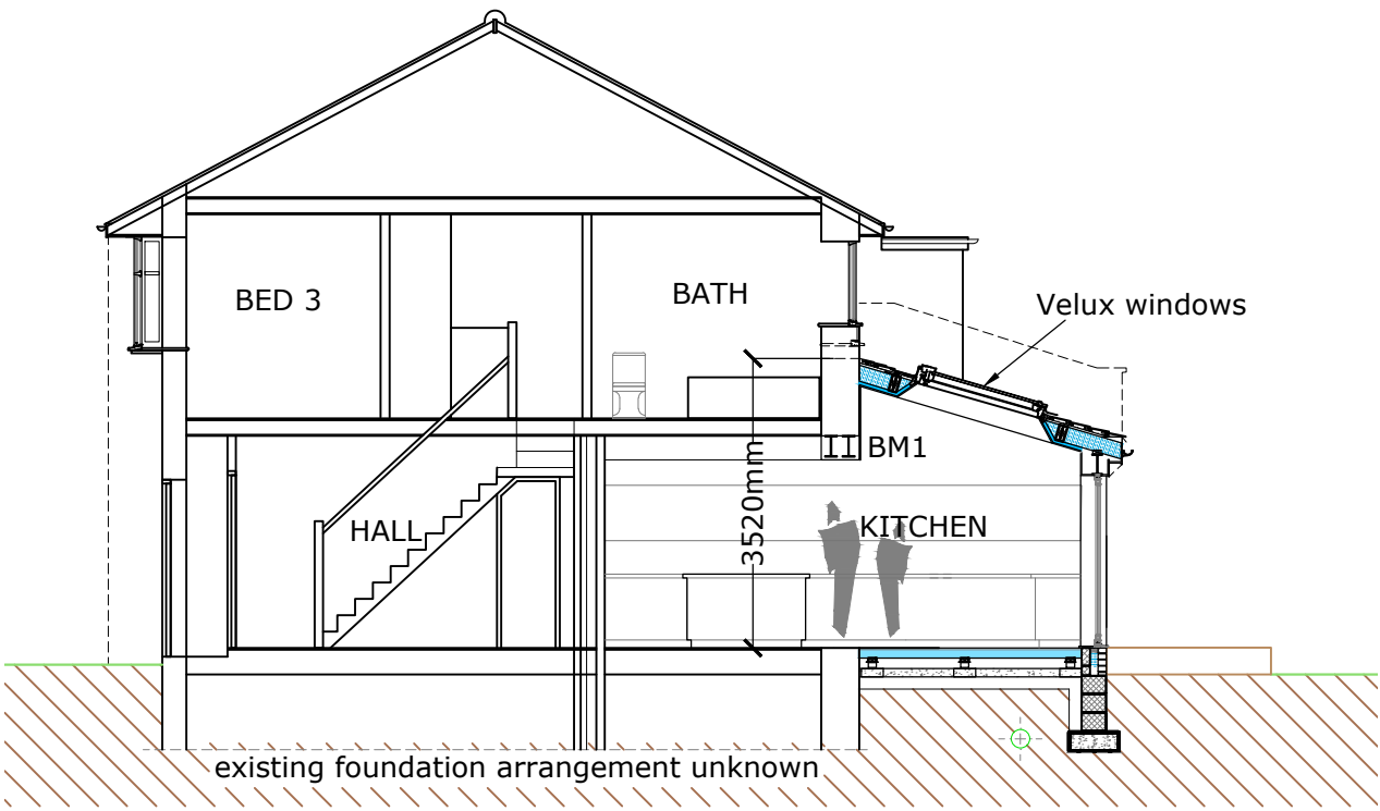
CROSS SECTION
