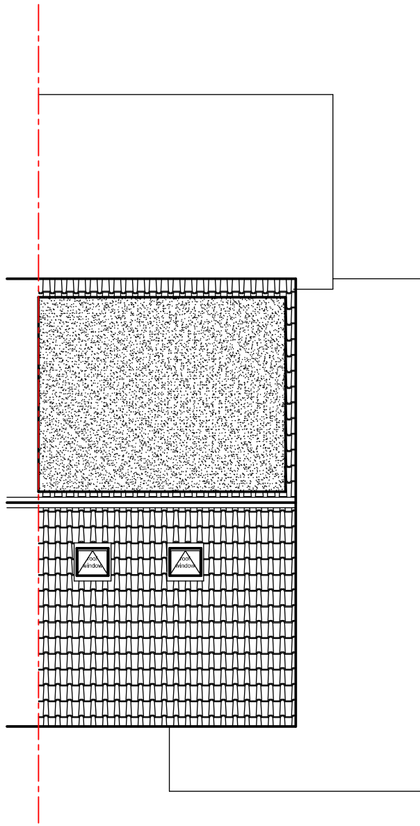
roof plan
