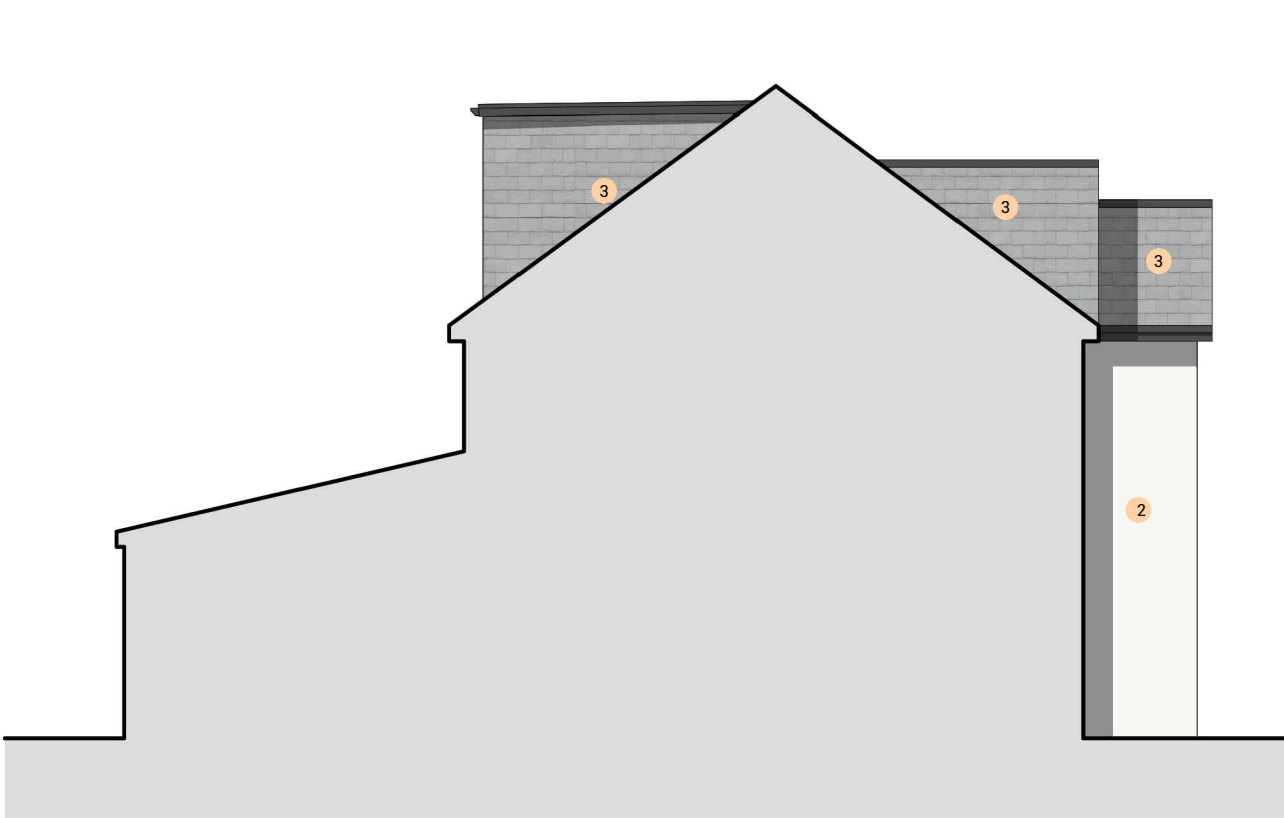
PROPOSED SIDE ELEVATION 1:100 @ A3
