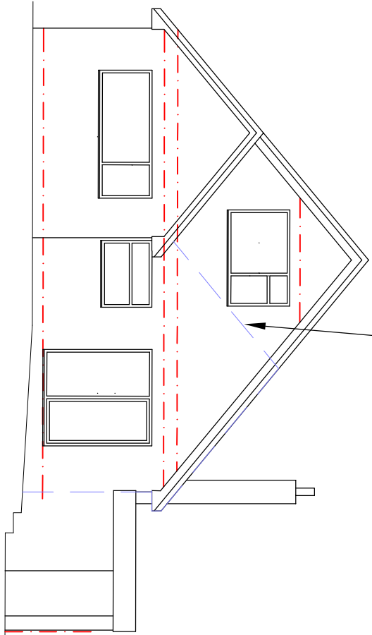
REAR ELEVATION 1:100
