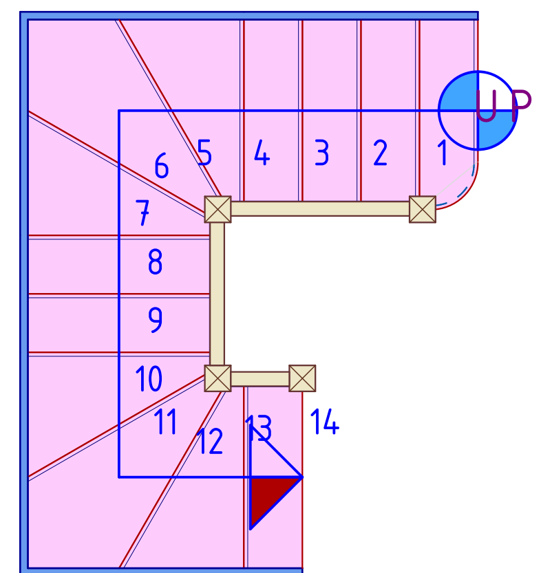
Stair Plan
