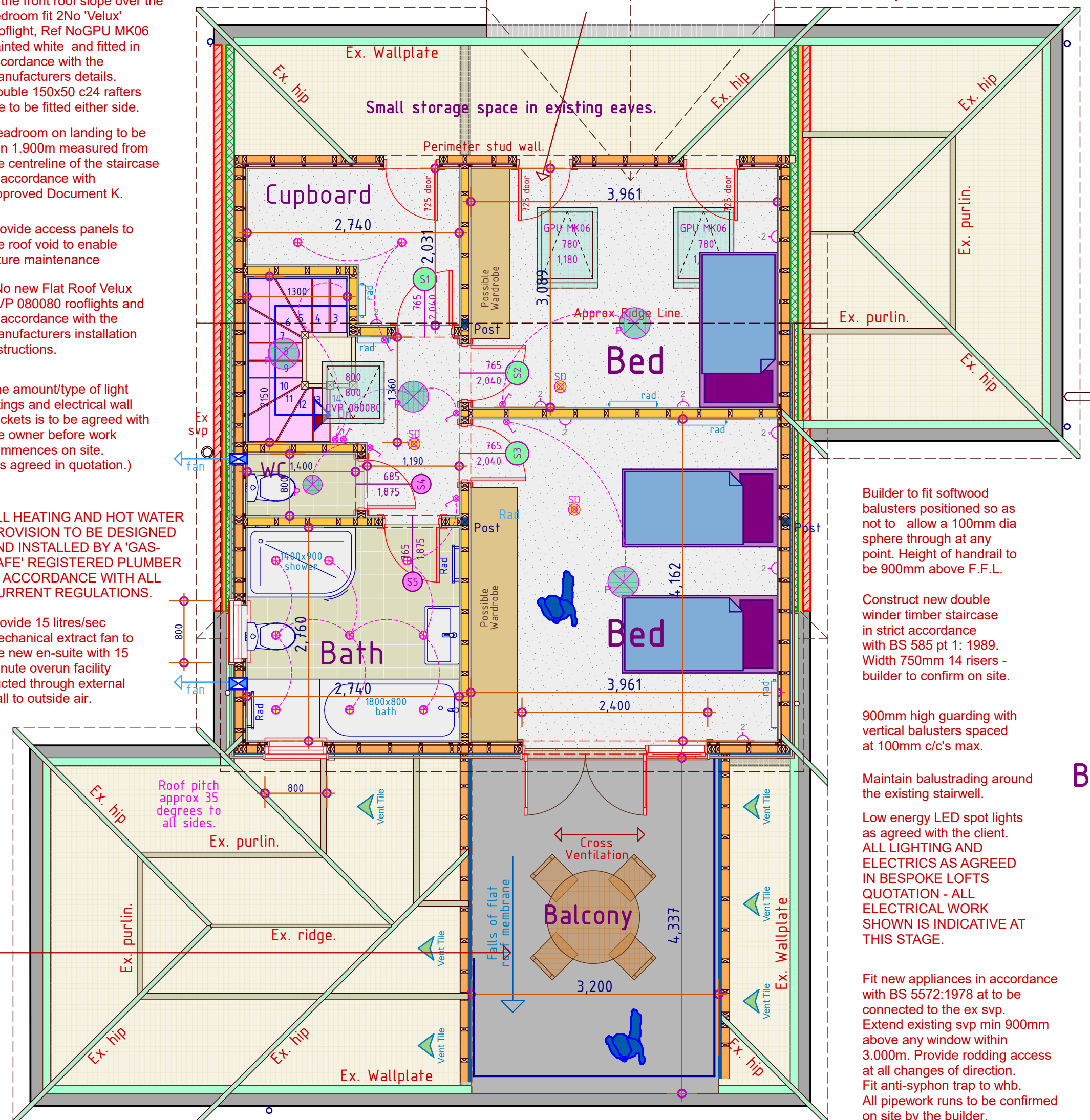
Proposed 2nd Floor Layout
