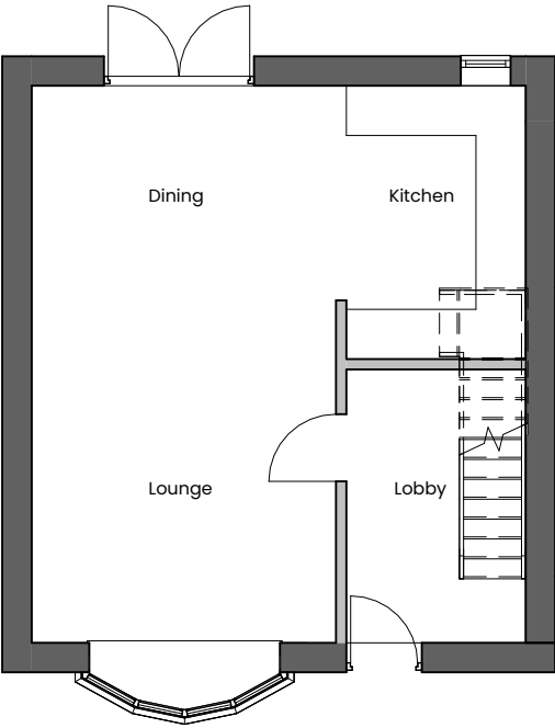
1 Existing Ground Floor 1 : 100
