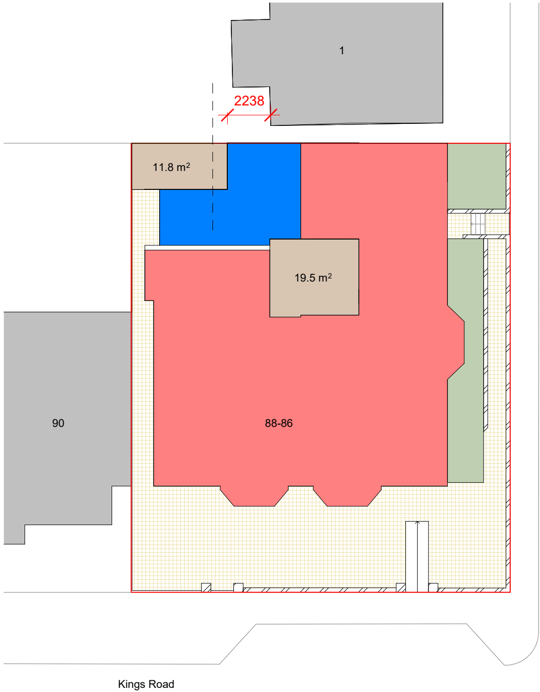
2 Site - Proposed 1 : 200
